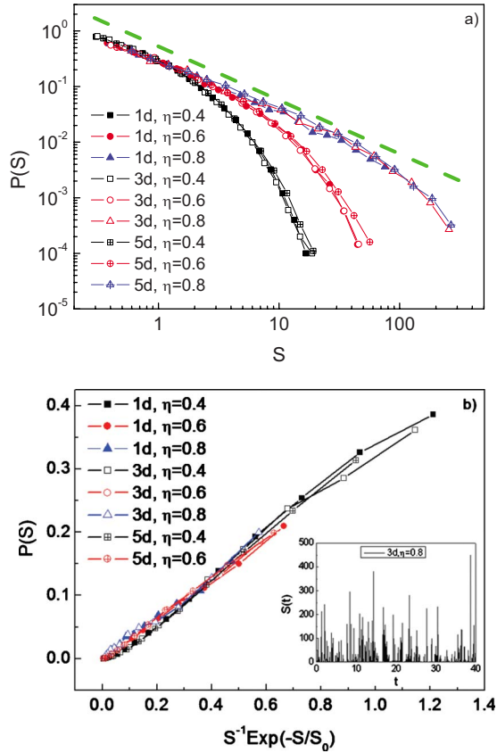
FIG. 2. (Color online) Probability density distribution functions of dislocation jump amplitudes for a single dislocation (1d) and for the central dislocation of packs of three (3d) and five (5d) dislocations. (a) curves showing the divergence of the cutoff size S_0 as the critical point \eta=1 is approached. The dashed line has slope -1 . (b) master curve obtained by normalization with S_0=1.03(1-\eta)^{-3.13} , S_0=1.07(1-\eta)^{-3.38} and S_0=1.13(1-\eta)^{-3.47} for 1d, 3d, and 5d, respectively. The inset shows part of a recorded signal for the 3d system with \eta=0.8 .
