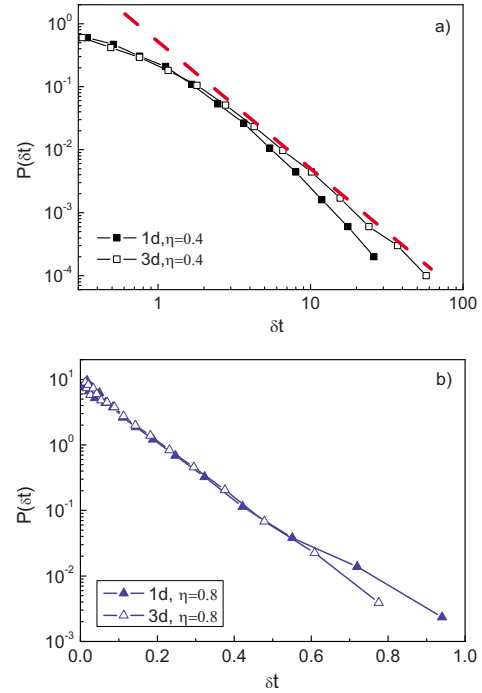
FIG. 3. (Color online) Probability distribution functions of wait times between unpinning events for a) \eta=0.4 (log-log plot) and (b) \eta=0.8 (semilog plot). The distribution is exponential at small \delta t and power law at large \delta t . The dashed line in (a) has slope -2 .
