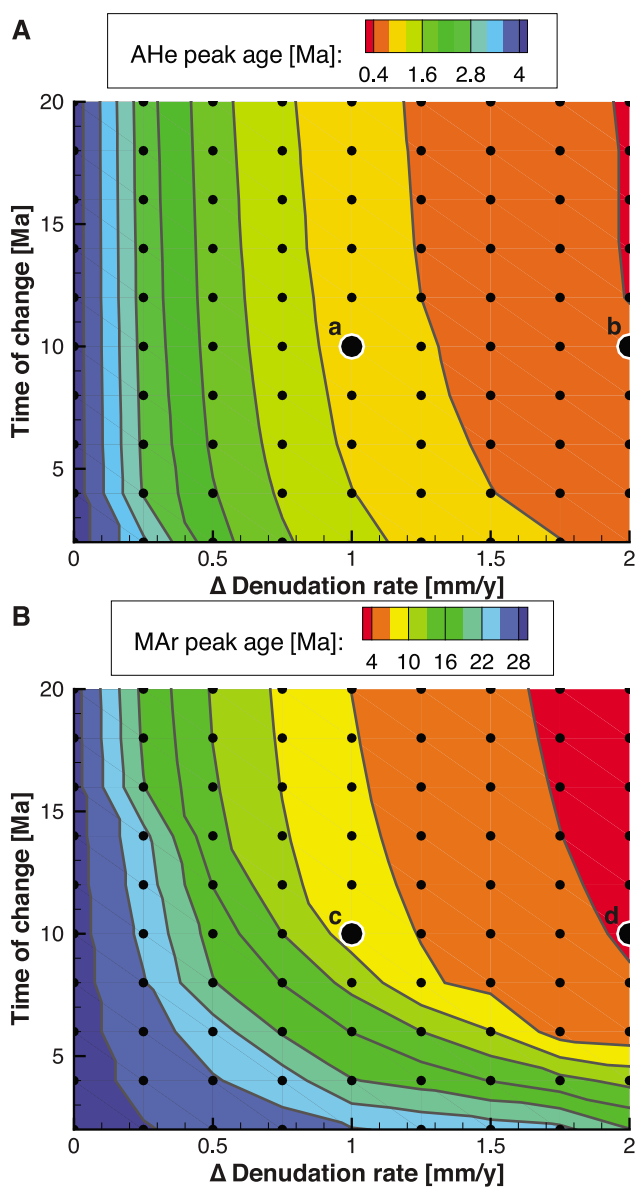
Figure 6. Changes in peak ages resulting from an acceleration in denudation rate at various times. The background denudation rate of 0.5 mm/y is accelerated by 0–2 mm/y at 2–20 Ma. Each small black circle represents an individual model run from which the contoured (a) AHe and (b) MAr peak ages were derived. The larger black circles are discussed in the text.
