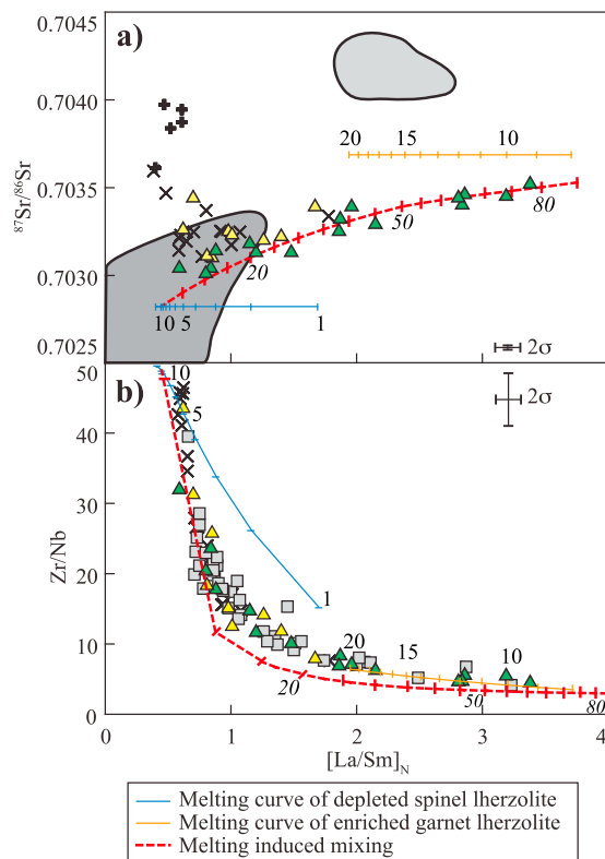
Figure 4. Geochemical characteristics of Group 2 lavas: (a) ^{87}\text{Sr}/^{86}\text{Sr} versus [\text{La}/\text{Sm}]_N and (b) \text{Zr}/\text{Nb} versus [\text{La}/\text{Sm}]_N . The standard deviation is 2\sigma . Mantle source composition, partition coefficients, and solid and liquid modes used for melting curve calculations are listed in Table 1. Our data are well reproduced considering the progressive dilution (from 60% to 0%) of the low-degree enriched melts ( F = 2\% ) in the aggregated liquids due to their mixing with melts issued from higher degree of melting ( F = 10\% ) of the depleted component. Symbols are as in Figure 3.
