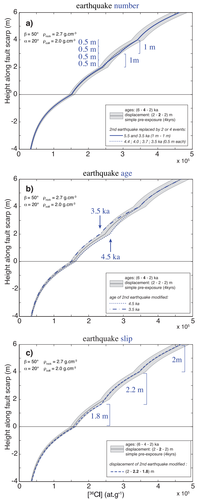
Figure 14. Effect of the variability in the earthquake number, age and slip on the ^{36}\text{Cl} production rates resulting in buried and exposed scarp rocks. Same reference curve as Fig. 12. (a) Each single large slip event may be a multiple event including several smaller events; small earthquakes cannot be discriminated. (b) Age differences lower than \sim 0.5 kyr cannot be discriminated. (c) Slip differences lower than \sim 0.2 m cannot be discriminated.
