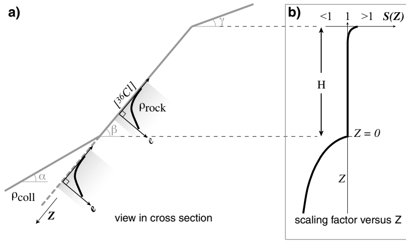
Figure A3. The attenuations along ‘ e ’ and ‘ Z ’ directions are separated: (a) the [Cl] profile due to rock attenuation is calculated for a surface of dip \beta in the direction e perpendicular, (b) a scaling factor S(Z) , which is only applied to the cosmogenic part of the production, is introduced. It accounts for both attenuation at depth ( S(Z) < 1 ) and increased flux at the vicinity of \gamma ( S(Z) ). It is calculated by scaling the cosmogenic production at surface far from \gamma (at Z = 0 , for \beta infinite).
