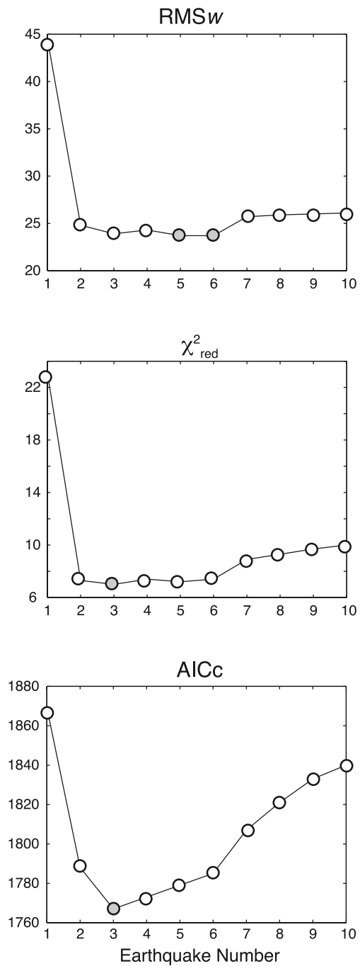
Figure 20. RMSw (weighted root mean square), \chi^2_{red} (Chi-square), AICc (Akaike Information Criterion with a second order correction) values obtained from fitting the Magnola data with 1–10 earthquakes (see text for details on fit indicators). Best values are obtained for 3–6 earthquakes. See Fig. 21 and Electronic Supplement 8 for the corresponding models.
