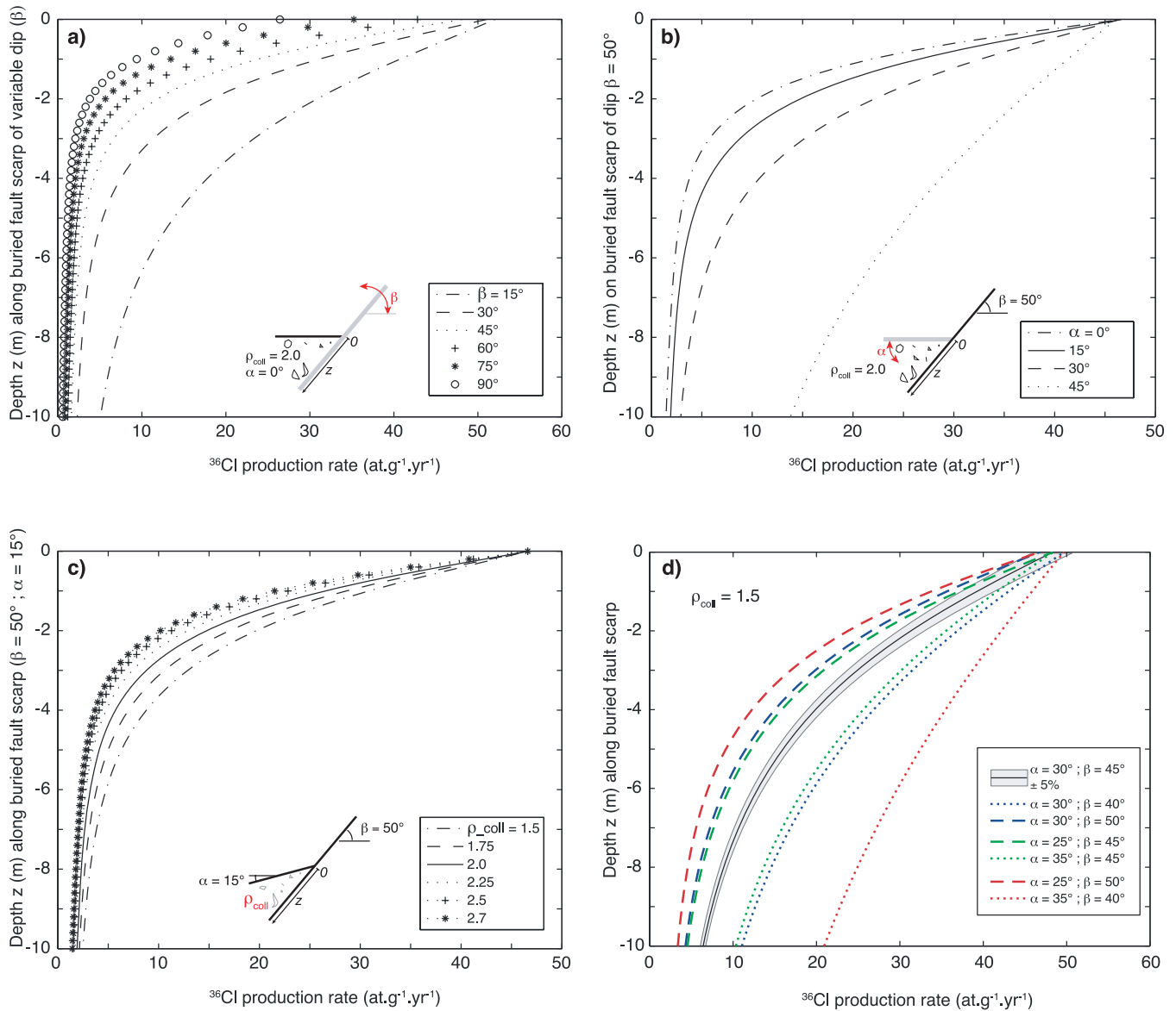
Figure 5. Effect of the fault scarp and colluvium geometry (dip) on the ^{36}\text{Cl} production rate ( \text{at.g}^{-1} \text{yr}^{-1} ) resulting in the buried fault scarp rocks (for a constant geomagnetic field). (a) Effects of the variations in the fault scarp dip ( \beta ). The colluvium is horizontal and of constant density ( \rho_{\text{coll}} = 2.0 \text{ g cm}^{-3} ). (b) Effects of the variations in the colluvium dip ( \alpha ). The fault scarp has a constant dip \beta = 50^\circ and the colluvium a density of 2.0 \text{ g cm}^{-3} . (c) Effects of the variations in colluvium density. The fault scarp and colluvium have a constant dip \beta = 50^\circ and \alpha = 15^\circ , respectively. (d) Combined effects of \pm 5^\circ uncertainty of the fault scarp and colluvium dips. A reference profile (continuous curve) is defined for common scarp and colluvium dip values ( \alpha = 30^\circ and \beta = 45^\circ ). The grey band represents the \pm 5 per cent uncertainty that would affect the reference profile, due to analytical measurement uncertainties. See discussion in text.
