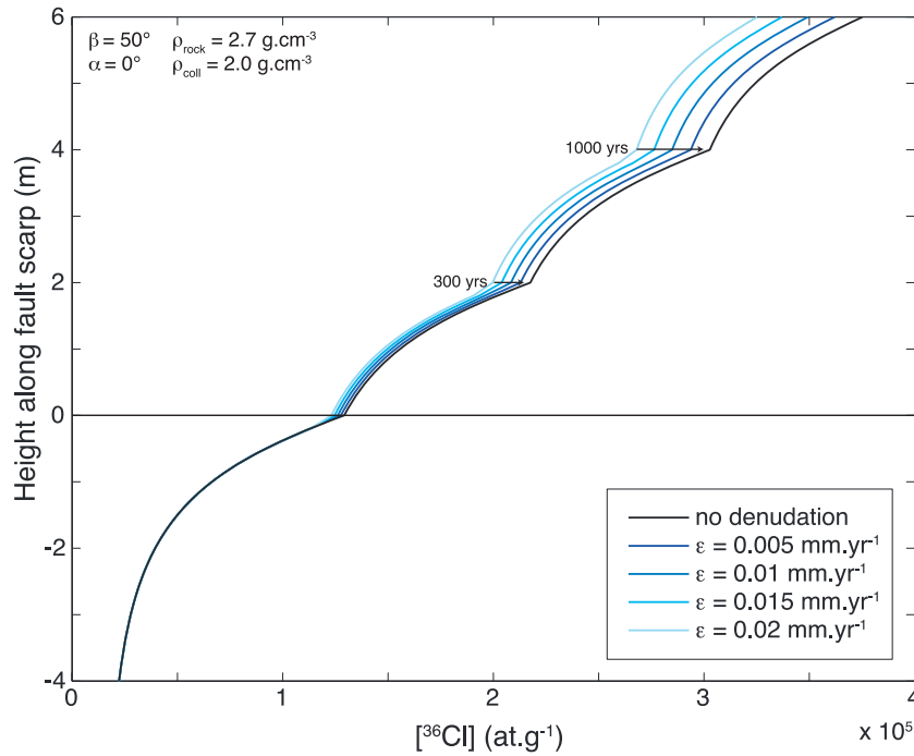
Figure 8. Effect of denudation on the [^{36}\text{Cl}] profile resulting in exposed scarp rocks. A reference curve is calculated for no denudation and 3 similar (2 m of on-fault slip), regular (every 2 kyr) earthquake exhumations. Ages are maximum age differences that are derived between the most extreme curves.
