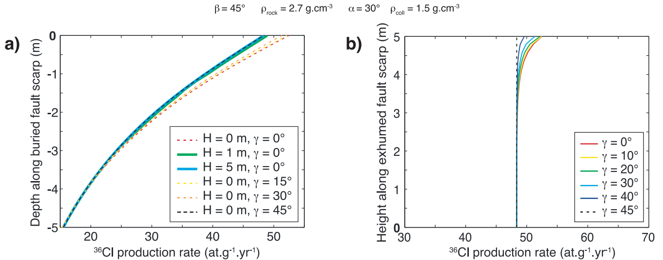
Figure 6. Effect of the upward shallowing of the fault scarp dip on the ^{36}\text{Cl} production rate (at g ^{-1} yr ^{-1} ) resulting in the buried and exposed scarp rocks (for a constant geomagnetic field; other parameters indicated on figure). The scarplet of dip \beta = 45^\circ shallows upward to a variable dip \gamma . H is height of the scarplet. (a) Effect of H and \gamma on buried samples. (b) Effect of proximity of \beta – \gamma slope break on exposed samples.
