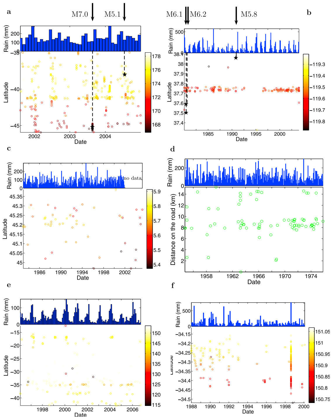
Figure 4. Space-time diagrams for landslide activity: landslides (circles) as a function of space (y axis for latitude and color for longitude) and time. The upper blue histogram gives monthly rainfalls (mm). The black arrows and black stars (New Zealand and Yosemite) give the location of the earthquakes which were reported in the catalog as having triggered landslides. (a) New Zealand, (b) Yosemite, (c) Grenoble, (d) Val d’Arly, (e) Australia, and (f) Wollongong. Figure 4d y axis corresponds to distances (km) along the road-cut.
