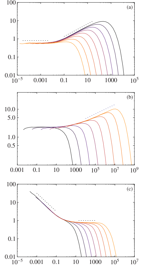
FIG. 3. (Color online) Normalized spectra for \nu=10^{-7} and \text{Pm}=1 . Curves (a) are shown for V_A=0 and \Omega=12.5, 25, 50, 100, 200, 400, 800 , and 1600 (from right to left, from darker to lighter). Curves (b) are shown for \Omega=0 and V_A=0.16, 0.32, 0.64, 1.28, 2.56, 5.12, 10.24 , and 20.48 (from left to right, from darker to lighter). Curves (c) are shown for (V_A, \Omega)=(0.16, 800); (0.32, 400); (0.64, 200); (1.28, 100); (2.56, 50); (5.12, 25); (10.24, 12.5); and (20.48, 6.25) (from left to right, from darker to lighter).
