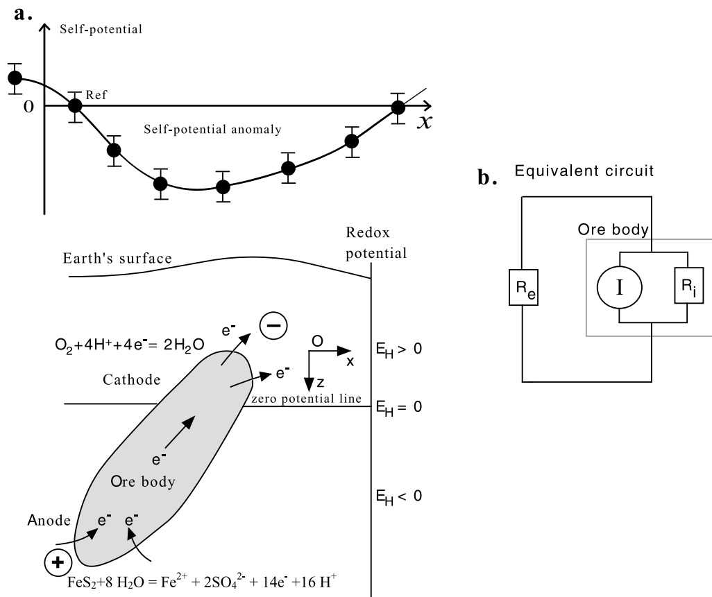
Figure 2. Sketch of the classical geobattery model proposed for ore bodies and equivalent linear circuit. (a) In the far field, the redox potential decreases with depth. In the vicinity of the ore body a disturbance of this far field is created because of the redox reactions at the surface of the ore body. Corrosion of the ore body can also be responsible for a resistive crust that adds an additional Ohmic resistance (and therefore an overvoltage) to the circuit. Typically, a self-potential anomaly associated with an ore body can amount to a few hundreds of millivolts at the ground surface but cannot be higher than the difference of the redox potential between the terminal points (anode and cathode) of the system. (b) The ore body is characterized by a source of current I and an internal resistance R_i . The resistance R_e stands for the external resistance of the conductive medium in which the ore body is embedded.
