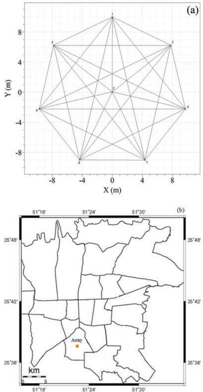
Figure 3. (a) Array configuration of the field experiment in southern Tehran. (b) Location of the array in the map of Tehran.
