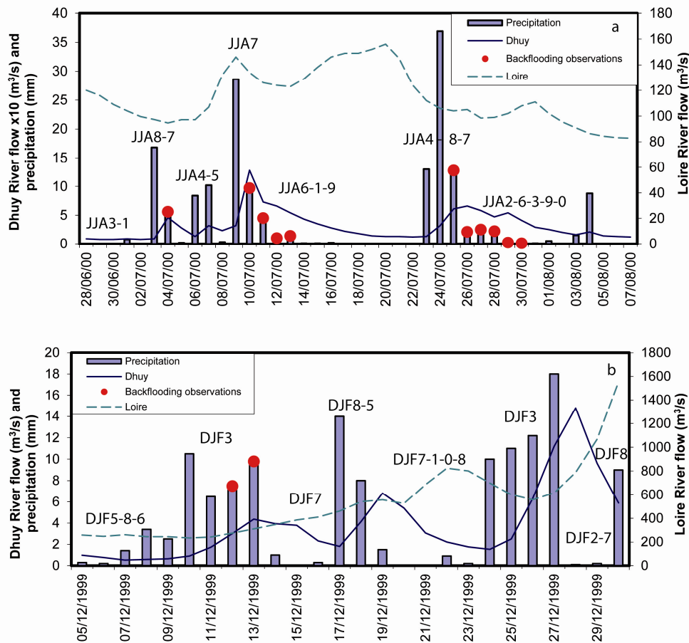
Fig. 6. Precipitations, Loire river flow, Dhuys river flow, backflooding observations and associated WT during a period of Loire stability (a) and a period of Loire high river flow (b).
