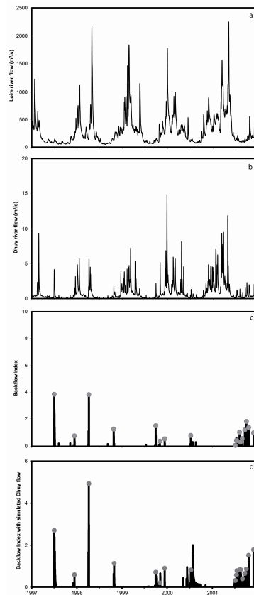
Fig. 3. Observed backflooding events and calculated backflow indices for 1997 to 2001. From the top down: Loire river flow ( a ), Dhuy river flow ( b ), backflow index calculated with the actual Dhuy river flows and the backflooding observations (grey circles) ( c ), backflow index calculated with the Gardenia-calculated Dhuy river flows and the backflooding observations (grey circles) ( d ).
