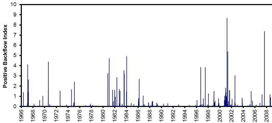
Fig. 4. Backflooding events between 1966 and 2009.
