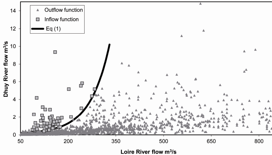
Fig. 2. Average daily Dhuys river flow versus the Loire river flow at Orléans between 1 June 1997 and 31 December 2001, with an indication of the outflow (triangles) and inflow (squares) functions of the karstic Bouillon Spring. Note: only Loire river flows below 850 m 3 s -1 are shown.
