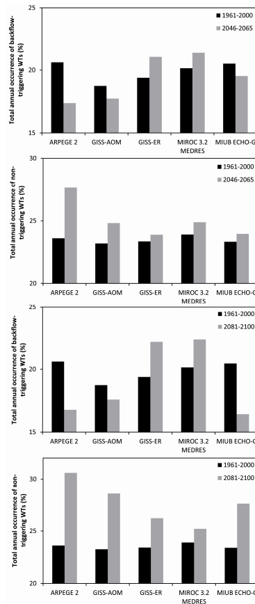
Fig. 9. Total annual occurrence (%) of backflow-triggering WTz (a) and non-triggering WTz (b) between the present and the near future and of backflow-triggering WTz (c) and non-triggering WTz (d) between the present and the distant future according to the five simulations.
