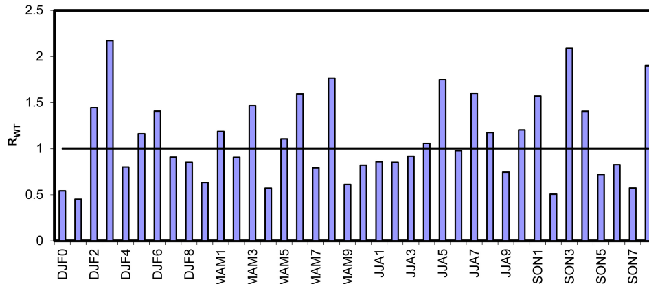
Fig. 5. Variability of the Dhuy river flow represented by the R_{WT} ratio for each weather type compared to the average seasonal flow. Note: R_{WT} = 1 corresponds to the average seasonal Dhuy river flow for the considered season.
