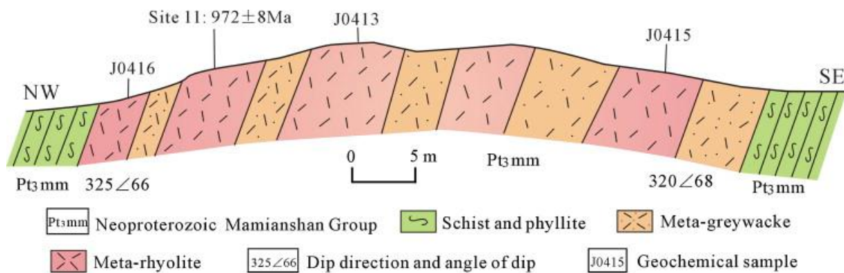
Fig. 7. Geological cross-section of the Jingnan area in the western segment of the Zhenghe–Dapu fault zone.
