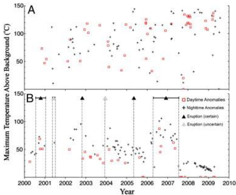
Fig. 10. Maximum temperatures above background for A) Erebus and B) Láscair. Red squares and black crosses denote daytime and nighttime images, respectively. The mid-point of eruptive episodes is denoted using a triangle symbol, the color of which indicates either high (i.e. black) or lesser (i.e. gray) levels of reported certainty in the occurrence of that eruption. When the start and stop date of an eruptive episode differ they are joined by a horizontal bar.
