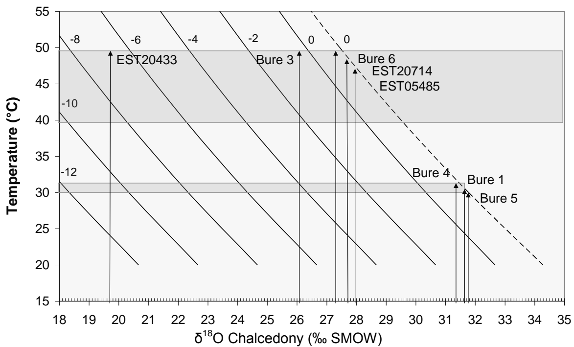
Fig. 15. T-\delta^{18}\text{O}_{\text{silica}} diagram in which are reported curves of temperatures in function of silica \delta^{18}\text{O} calculated at equilibrium with fluids whose \delta^{18}\text{O} are 0, -2, -4, -6, -8, -10, -12 ‰ (SMOW). Grey areas correspond to temperature ranges of chalcedony formation in the Callovian-Oxfordian formation. Low temperatures around 30°C may correspond to beginning of burial, whereas 40-50°C range corresponds to the maximal burial of the clay formation.
