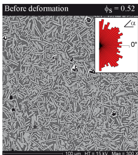
Figure 1. SEM microphotograph of a plagioclase bearing suspension before deformation with \phi_s = 0.52 . Plagioclase in light grey, silicic glass in dark grey and gas bubbles in dark. The inset shows the local plagioclase fabric long axis orientations ( \alpha ) displayed together on the rose diagram. Long axis orientations \alpha are respectively positive and negative for an counterclockwise and a clockwise orientation.
