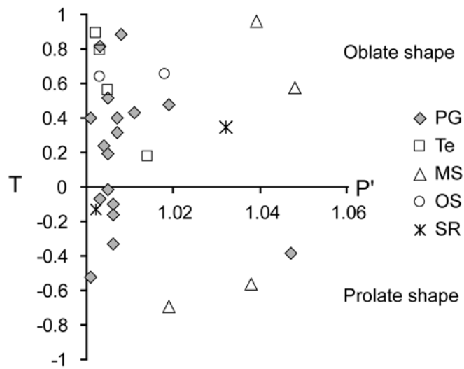
Figure 6. Graphic presentation of the shape parameter T versus the corrected anisotropy degree P' for all sites. PG: primary gossans, MS: massive sulfides, OS: oxidized stockworks, SR: surrounding rocks, Te: terraces.
