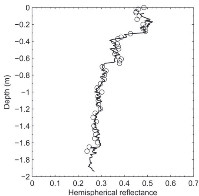
Fig. 9. Profiles of hemispherical reflectance measured with POSSUM (solid line) and discontinuous measurements with DUFISSS (circles) obtained on Glacier de la Girose on 17 April 2009.
