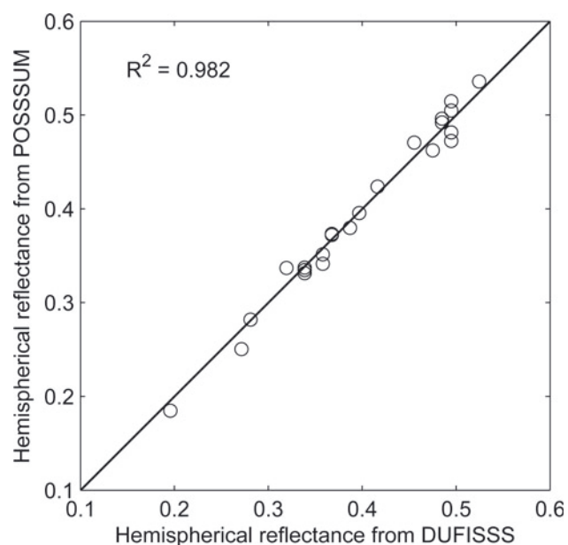
Fig. 8. Comparison of hemispherical reflectances obtained in the laboratory using snow samples with POSSUM and DUFISSS (circles). R^2 is computed with the residual sum of squares errors between the real data points and the y=x model.
