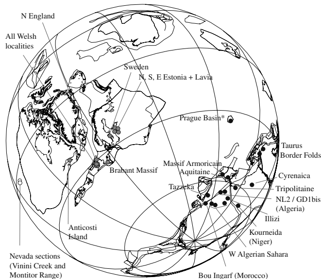
Fig. 2. Hirnantian paleogeographical reconstruction (27). The shading represent TWINSPAN clusters, i.e. Polar (black), Tropical (white), and Subpolar to Subtropical localities (gray; SI Materials and Methods ). *We do not follow this reconstruction for the Prague Basin on the wandering Perunica “micro-continent,” which is shown to have been at higher paleolatitudes (31).
