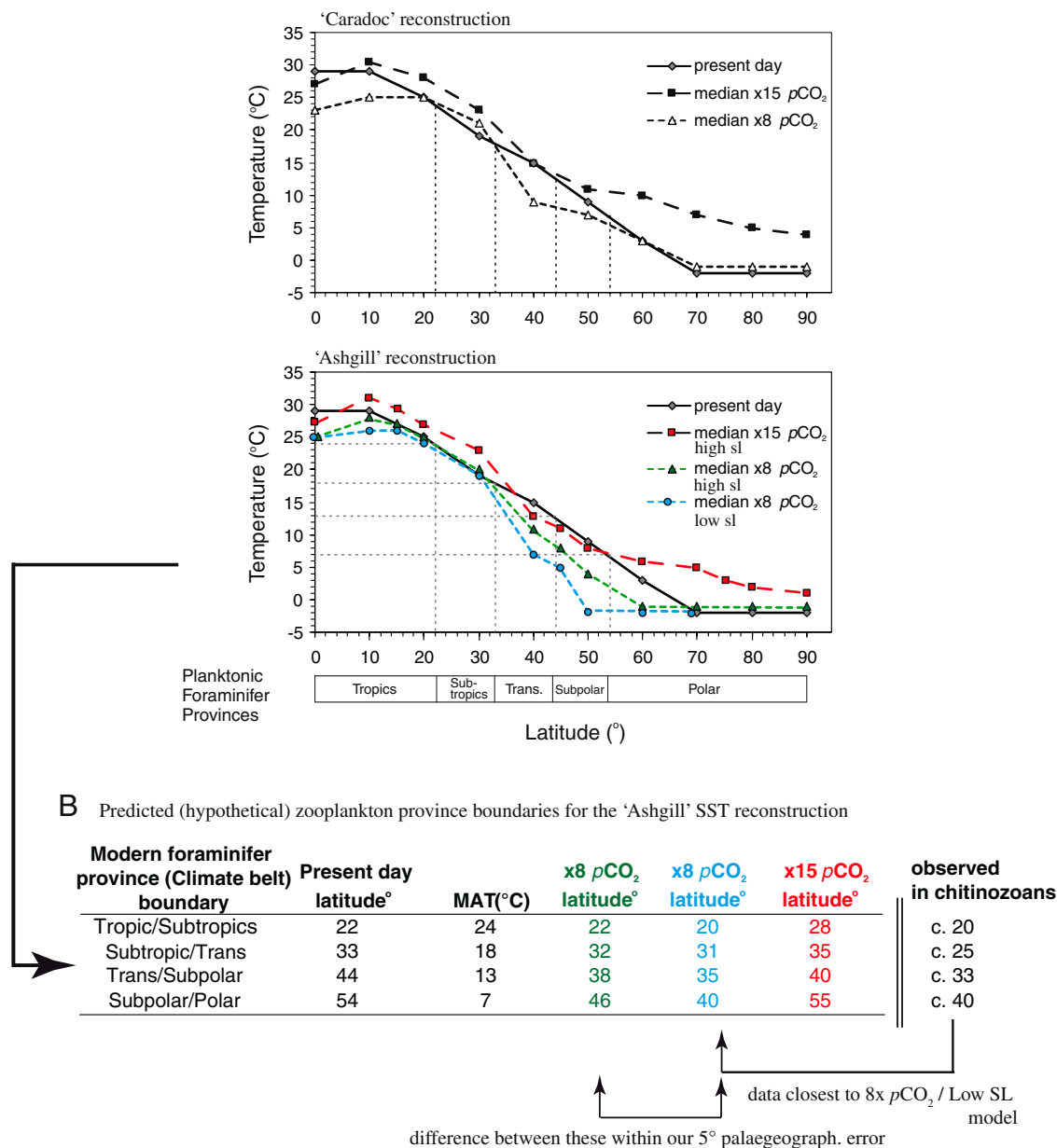
Fig. 1. Model predictions. (A) Latitudinal SST gradients and profiles from Sandbian and Hirnantian (Caradoc and Ashgill) SST models (x8 and x15 PAL pCO 2 ) (5) compared with present-day SST (ref. 30, central Pacific Ocean, taken from http://www.noaa.gov ). Modern day planktonic foraminifer provinces in terms of SST (29). (B) Using SST simulations of Herrmann et al. (5) at x8 (high sea level/low sea level) and x15 PAL pCO 2 we estimate the position of these zooplankton provinces/belts and their boundaries during the Hirnantian, for different pCO 2 scenarios. MAT: mean annual temperature.
