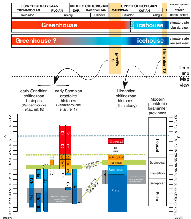
Fig. 4. Late Ordovician Polar Front migration. Time line showing a Katian (2) start of Late Ordovician cooling and a revised view with an earlier onset (15). Our Sandbian data (17, 18) support the latter. The map view compares Sandbian and Hirnantian chitinozoan biotopes; these maps demonstrate an equatorward shift in the position of the Polar Front from 55^\circ to 70^\circ S to likely 40^\circ S, which involves an equatorward incursion of Polar water and a compression of the Subpolar belt and fauna (diversity). The subtropical belt moves slightly northwards. The shift of the Polar Front maps onto well-known patterns of late Cenozoic glacial-interglacial Polar Front migration.
