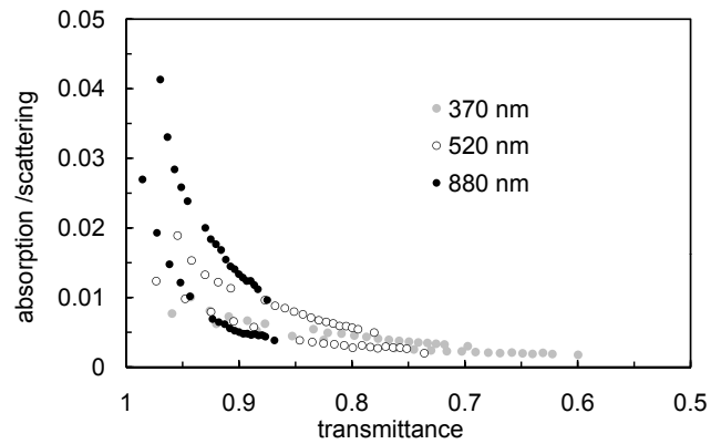
Fig. 11. Sensitivity to particle scattering as a function of filter transmittance for the 7 \lambda -Aethalometer. Shown are the ratios of absorption coefficients divided by scattering coefficients for three wavelengths. Absorption coefficients were corrected using Weingartner et al. (2003).
