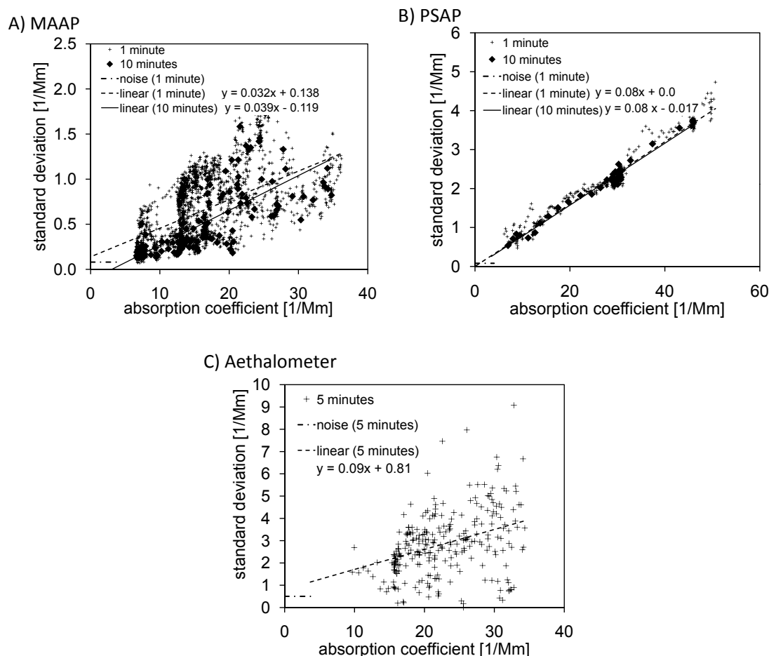
Fig. 9. EUSAAR2007: Unit to unit variability (standard deviation of several instruments) vs. absorption coefficient for (a) MAAP (seven instruments), (b) PSAP (six 3\lambda -PSAP, green) and (c) Aethalometer (four 7\lambda -Aethalometers, 660 nm). PSAP and MAAP data are shown for the highest time resolution of one minute and for an averaging time of ten minutes. Aethalometer data are shown for an averaging time of 5 min. The noise level is indicated as horizontal line.
