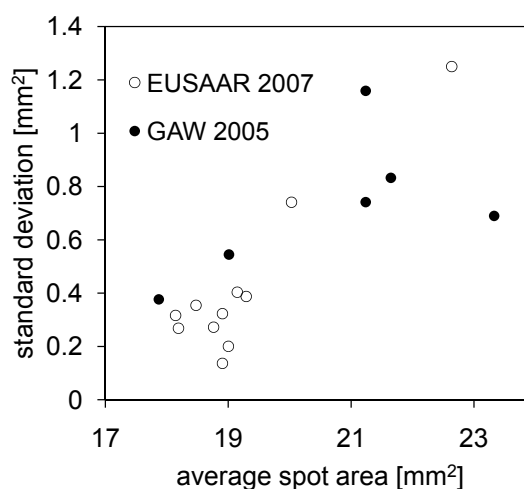
Fig. 5. Standard deviation of PSAP spot area versus average spot area. Each point is for one PSAP. The nominal spot area given by the manufacturer is 17.85 \text{ mm}^2 .
