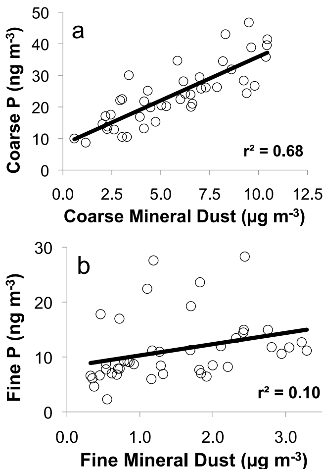
Figure 7. Linear regression analysis showing the significant positive correlation exhibited between (a) coarse atmospheric TP and mineral dust concentration. (b) This correlation was much weaker in fine PM samples.
