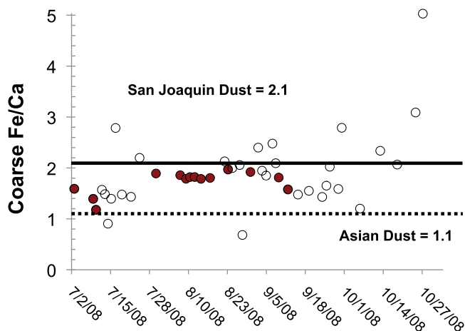
Figure 5. Temporal variability in the Fe/Ca mass ratio of coarse PM samples collected at the Lower Kaweah site showing the significant increase over background levels in October. Samples characterized by high mineral dust loading ( >7 \mu\text{g m}^{-3} ) are indicated with solid dots.
