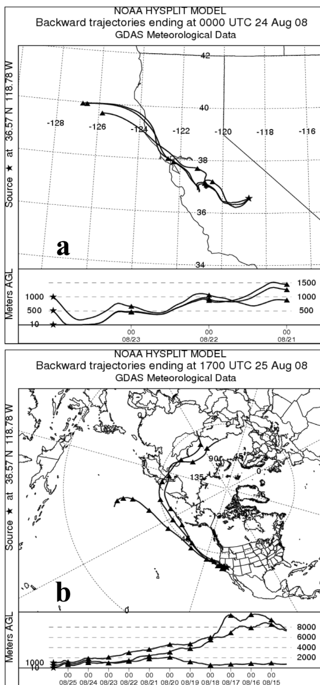
Figure 2. (a) Three day and (b) 11 day backward trajectories of the air masses reaching the Lower Kaweah site in late August, showing the most common regional and long-range transport patterns, respectively. AMBT data was obtained from the National Oceanic and Atmospheric Administration (NOAA) GDAS database using the hybrid single-particle Lagrangian integrated trajectory (HYSPLIT) model [Draxier and Hess, 1998] and is described in greater detail by Vicars et al. [2010]. AMBTs were calculated at 10, 500, and 1000 m above ground level.
