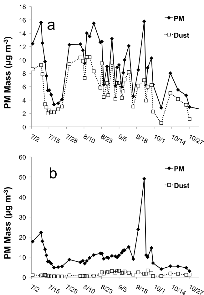
Figure 3. Temporal variability in total PM and estimated dust mass concentrations for (a) coarse and (b) fine filter samples.
