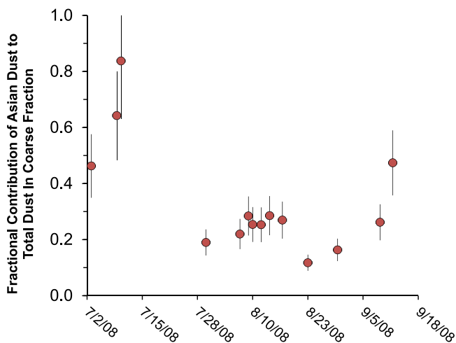
Figure 6. Fractional contribution of Asian dust sources to total dust in the coarse aerosol fraction computed from a two-component mixing model incorporating Asian and San Joaquin Valley dust end-members. Data shown are from samples characterized by high mineral dust loading ( >7 \mu\text{g m}^{-3} ). Error bars denote the 95% confidence interval for the Asian dust contribution.
