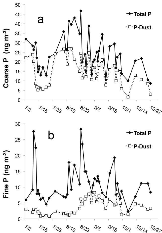
Figure 8. Temporal variability in total P and estimated P dust concentrations for (a) coarse and (b) fine filter samples.
