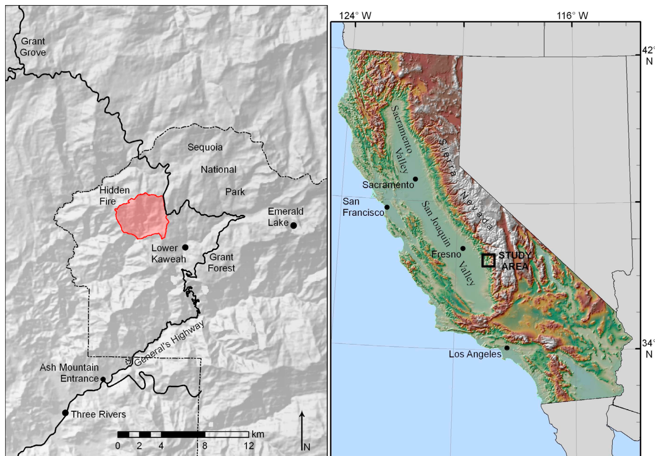
Figure 1. Map of California and location of the Lower Kaweah sampling site in the southern Sierra Nevada.
