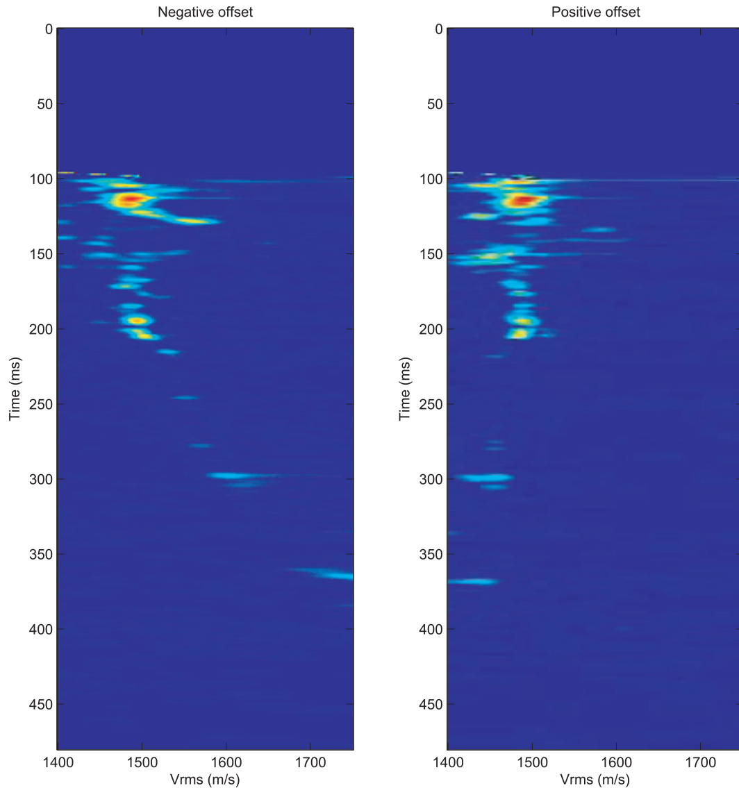
Figure 7. Semblance analysis performed on OBH 3. The OBH data were split in two sets (positive and negative offsets). A quasi-constant velocity characterizes the first 200 ms below the seabed. After 200 ms, one can observe the difference in the velocity estimate.
