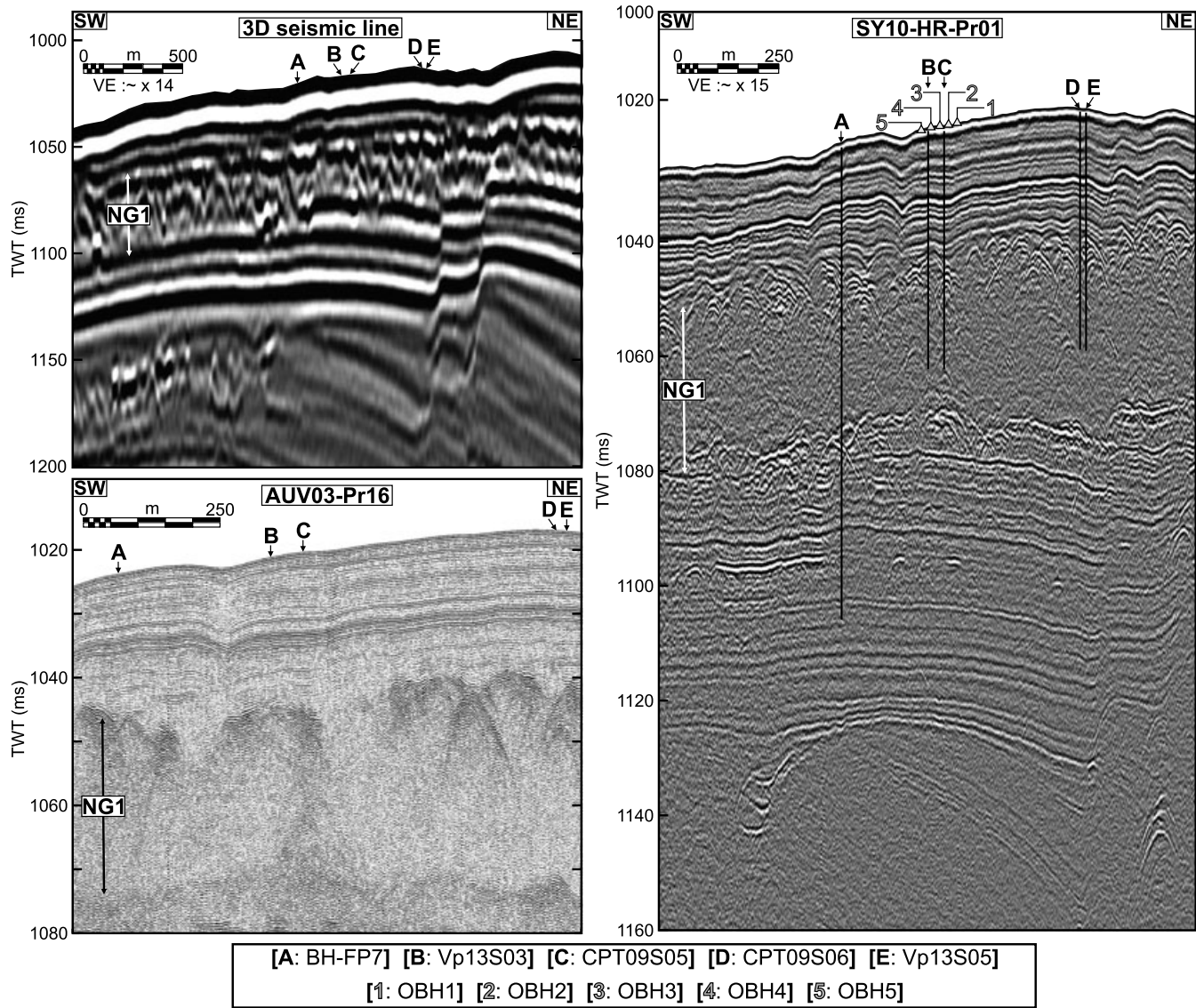
Figure 12. Top left-hand side: seismic line extracted from a 3-D cube. Bottom left-hand side: AUV sub-bottom profiler line (1800–5000 Hz). Right-hand side: SYSIF line (220–1050 Hz).
