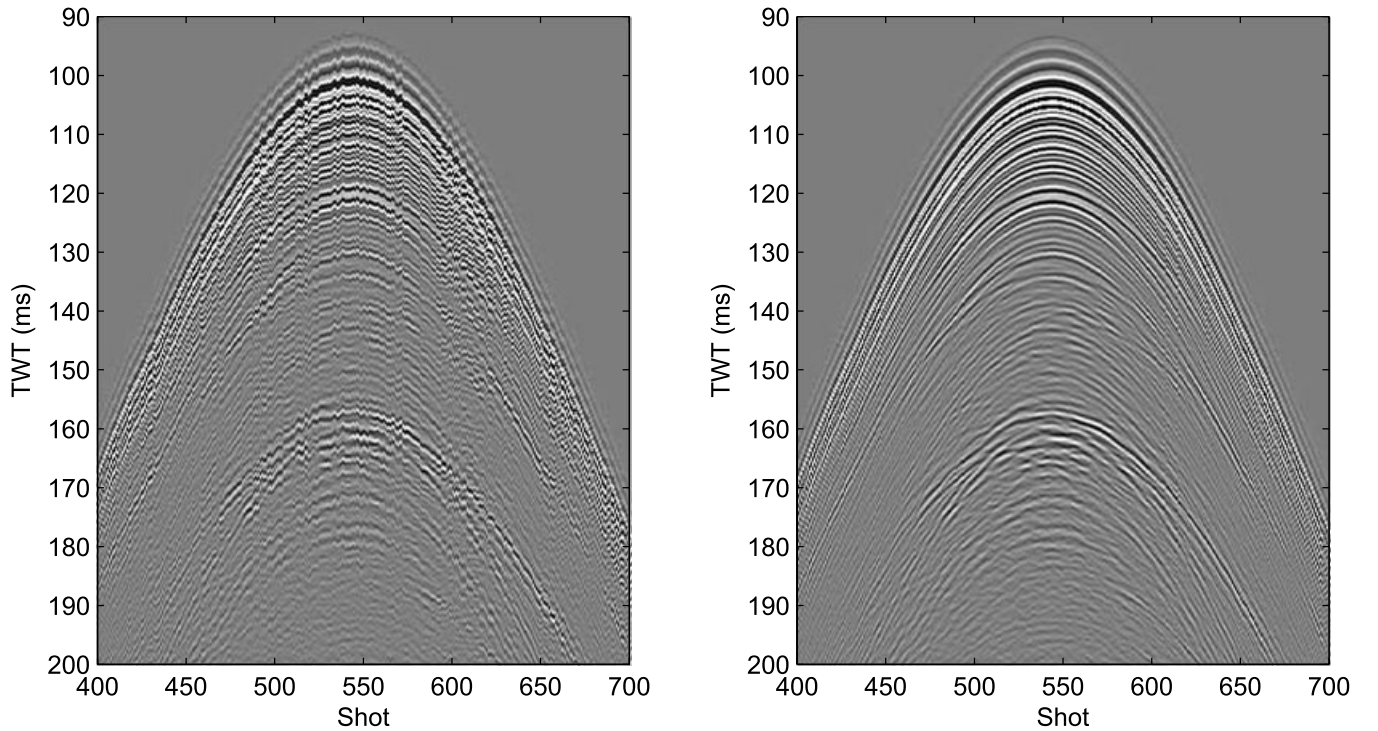
Figure 3. OBH 3 before (left-hand panel) and after (right-hand panel) the correction of the jitter related to the source position variations.
