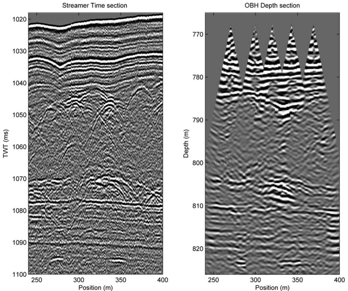
Figure 10. Comparison between the streamer time section and a stack of OBH depth images.
