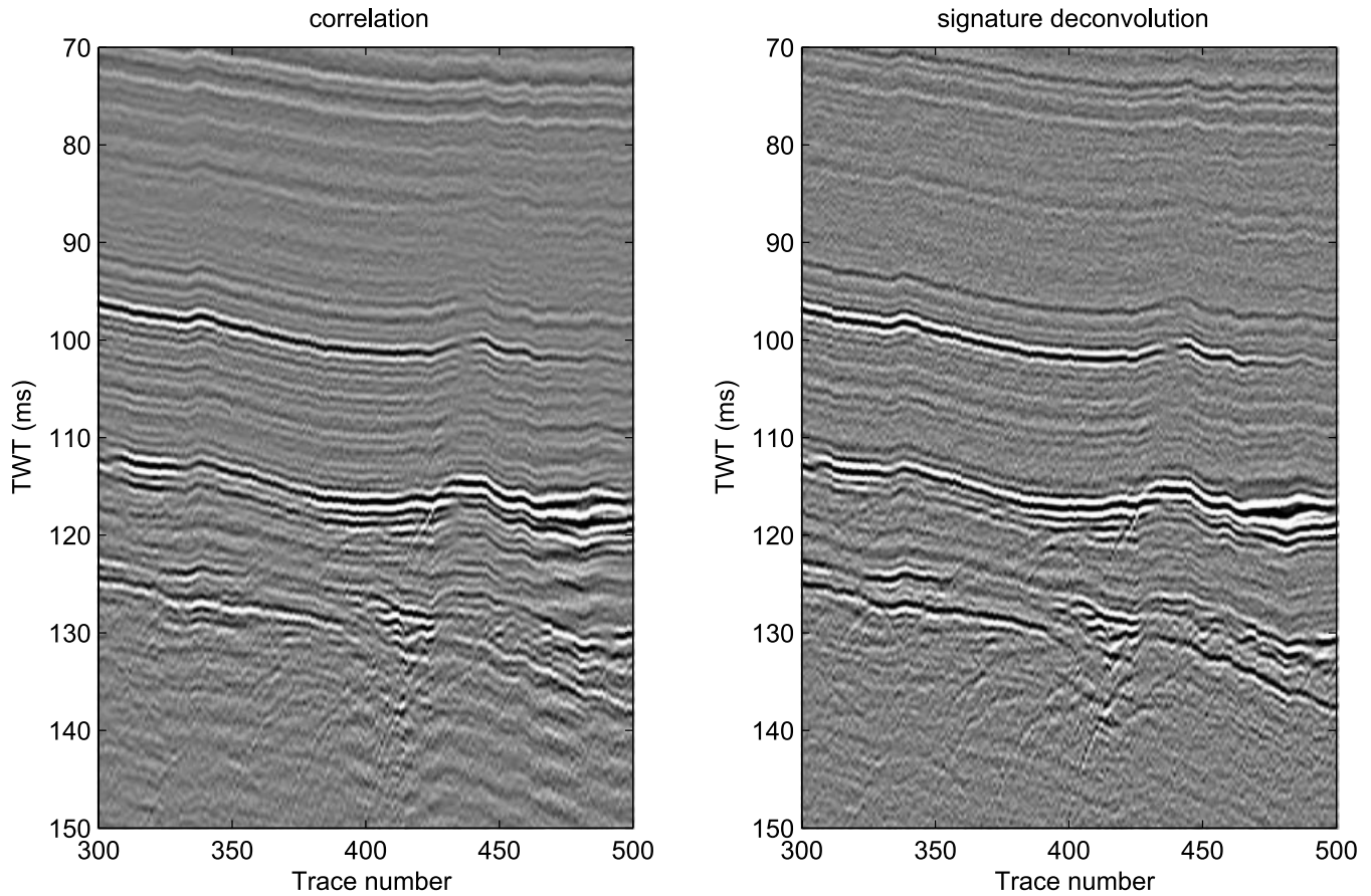
Figure 6. Left-hand panel: correlation processing (filter 350–1100 Hz). Right-hand panel: deconvolution processing (filter 200–1100 Hz).
