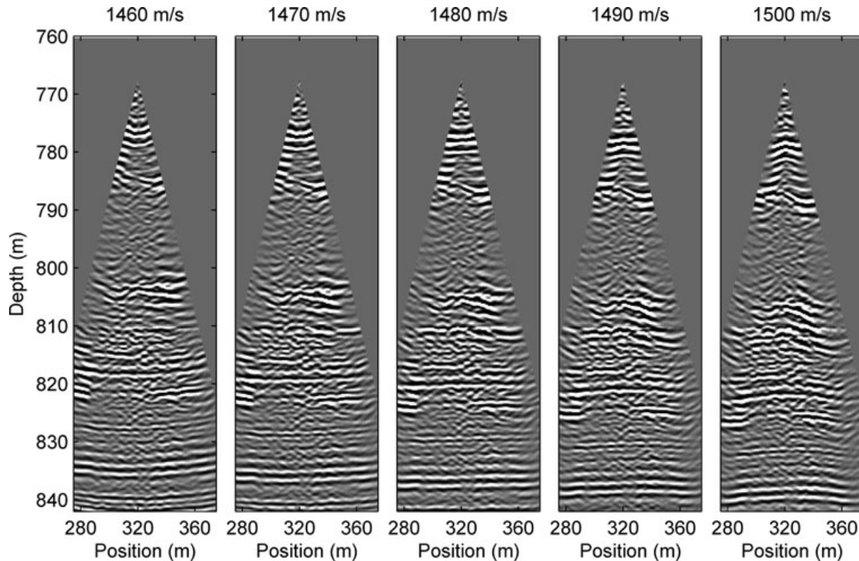
Figure 8. Velocity scan performed on OBH3. OBH3 was migrated with close constant velocities (1460, 1470, 1480, 1490 and 1500 ms). The change in shape of reflectors unveils sensitivity finer than 10 \text{ m s}^{-1} . A velocity of 1480 \text{ m s}^{-1} ensures the correct depth migration of the shallow part of the section (up to 840 m) which includes the MTC NG1.
