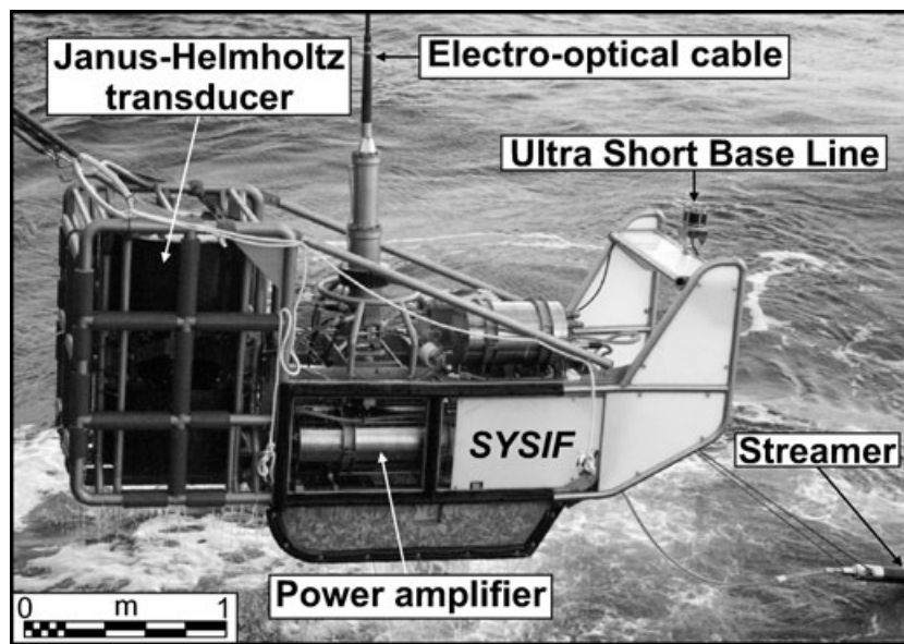
Figure 2. Picture of the SYSIF heavy-towed vehicle during a JH250-6000 deployment.
