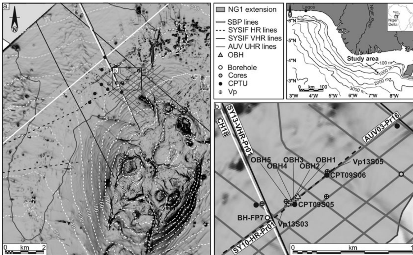
Figure 1. (a) Seabed dip map showing in grey the areal extension of the distal part of NG1. Location of the seismic data, cores and in situ measurements collected during the ERIG3D cruise. (b) Close-up of the location map showing the data used in this study.
