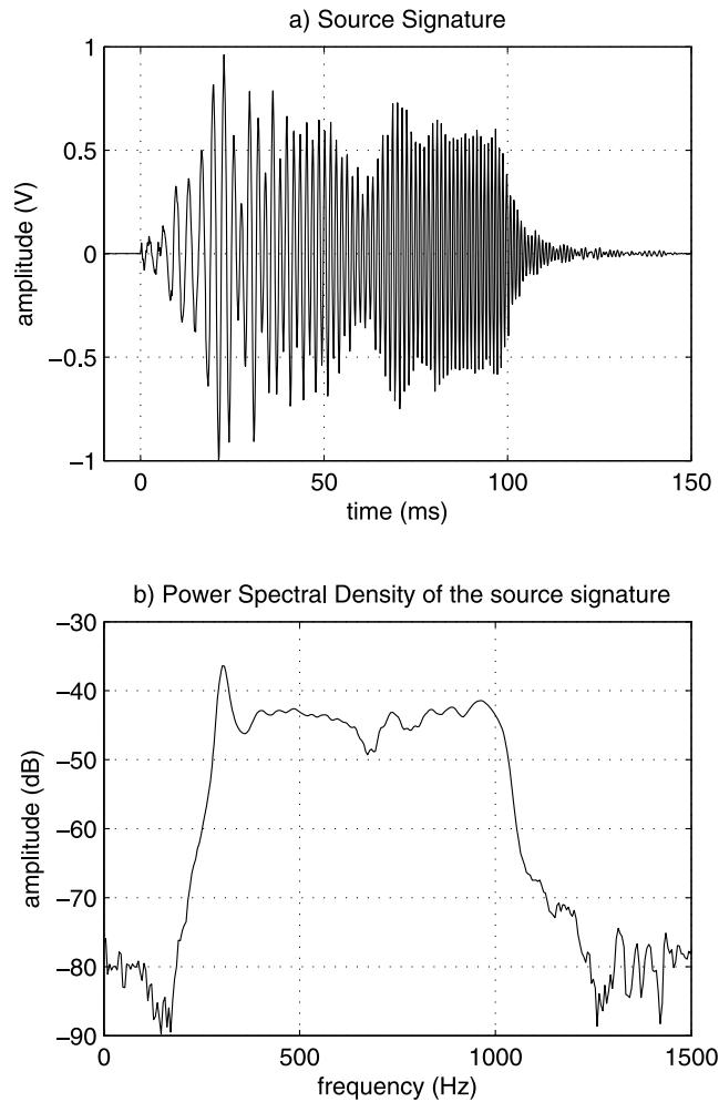
Figure 5. (a) Mean source signature recorded in far field condition. (b) Power spectral density of the source signature.
