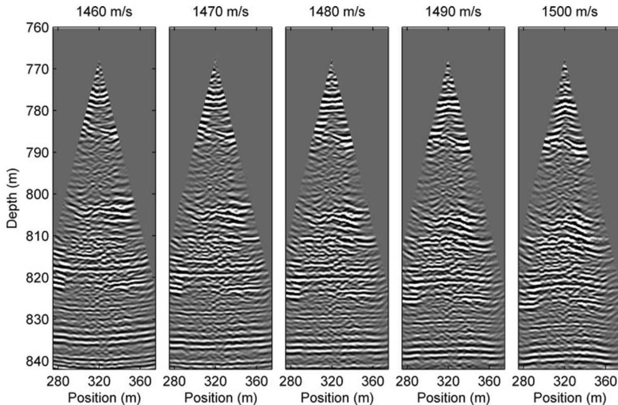
Figure 8. Velocity scan performed on OBH3. OBH3 was migrated with close constant velocities (1460, 1470, 1480, 1490 and 1500 ms). The change in shape of reflectors unveils sensitivity finer than 10 \text{ m s}^{-1} . A velocity of 1480 \text{ m s}^{-1} ensures the correct depth migration of the shallow part of the section (up to 840 m) which includes the MTC NG1.
