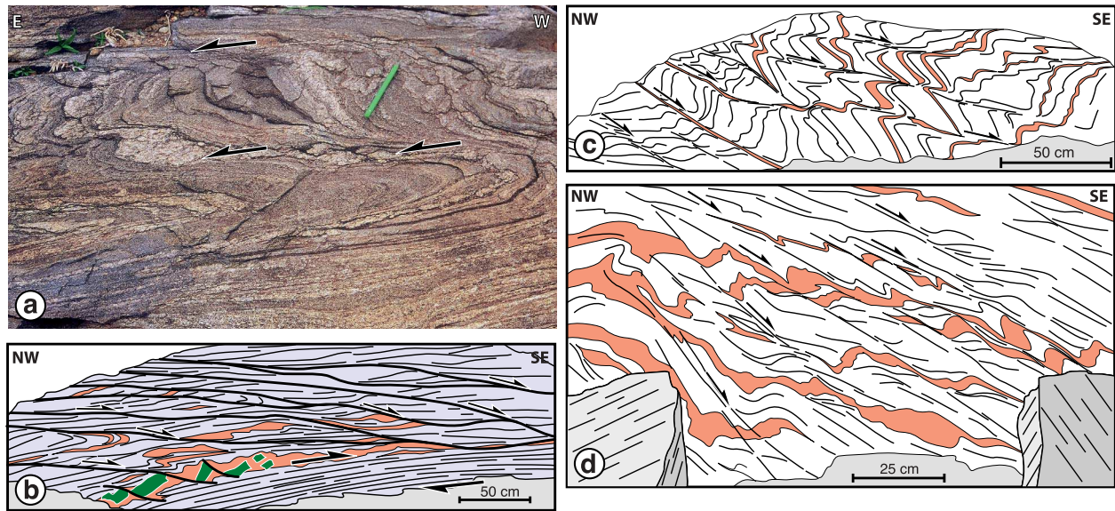
Figure 6. Fold and shear patterns in the eastern gneisses. (a) Similar folds in unit b, 3 km north of Rolla. (b) Low-angle synmetamorphic shear zones in unit b, between Agrahara and Agali (on the trace of a map-scale NE trending shear zone; Figure 5). (c) Relations between folds and shear zones, unit a, 5 km west of Agali. (d) Shear bands and related folds in fabric-free leucocratic veins, unit a (locality of sample CL20A). Leucosomes or granitic veins or felsic gneissic layers are shown in red and amphibolites in green. Sketches are line drawings of field photographs. See Figures 3 and 5 for locations and terminology of the units.
