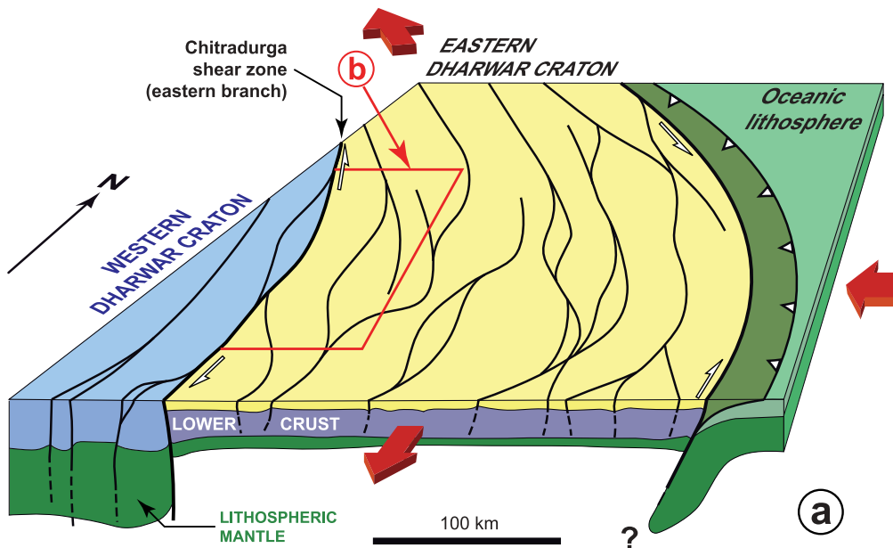
Figure 11. (a) Configuration of the Neoproterozoic orogen of south India between 2.56 and 2.50 Ga. The eastern edge of the orogen may be tentatively seen as a westward dipping subduction. Transient mechanical decoupling along this subduction could have resulted in synconvergence eastward spreading of the orogen, which would explain the systematic east side down transtensional component of lateral constrictional flow (e.g., Figure 7). (b) Textural and compositional fabric pattern of the central part of the Neoproterozoic orogen. The red box corresponds to the block diagram of Figure 9a. A tentative comparison is suggested between the crustal texture of the Eastern Dharwar craton and the INDEPTH III reflection seismic data (c) from the Bangoin shot in central Tibet (adapted from Ross et al. [2004]).
