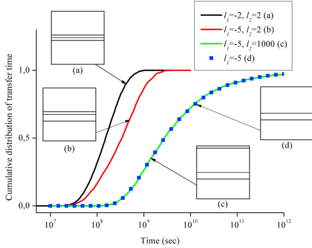
Figure 2. Cumulative distribution of the transfer time to nearby fractures. Particles transfer from position x = 0 to positions x = l_1 and x = l_2 . Solid lines and dots represent results obtained with Feller and FPTD formulations, respectively. The local diffusion coefficient is equal to 10^{-8} m 2 /s, and the fracture positions are expressed in meters.
