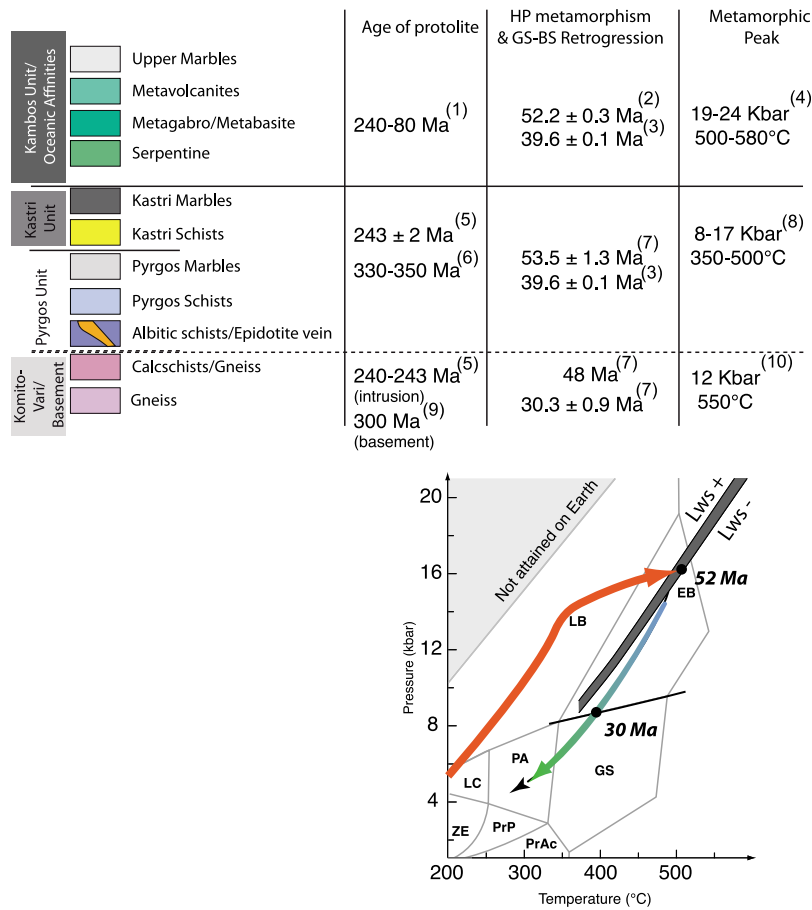
Figure 2b. Geological pile on Syros Island showing the ages of the protolite, metamorphism, and blueschist (BS) to greenschist transition (GS). Superscript numbers indicate the following citations: (1) Bulle et al. [2010], (2) Lagos et al. [2007], (3) Baldwin [1996], (4) Holley et al. [2004], (5) Keay [1998] and Tomaschek et al. [2003], (6) Pohl [1999], (7) Maluski et al. [1987], (8) Schumacher et al. [2008], (9) Tomaschek et al. [2008], and (10) Tomaschek and Ballhaus [1999]. Geochronological data are plotted in the PT path after Schumacher et al. [2008]. Facies are EB, epidote-blueschist; GS, greenschist; LB, lawsonite blueschist; LC, lawsonite-chlorite; PA, pumpellyite-actinolite; PrAc, prehnite-actinolite; PrP, prehnite-pumpellyite; and ZE, zeolite.
