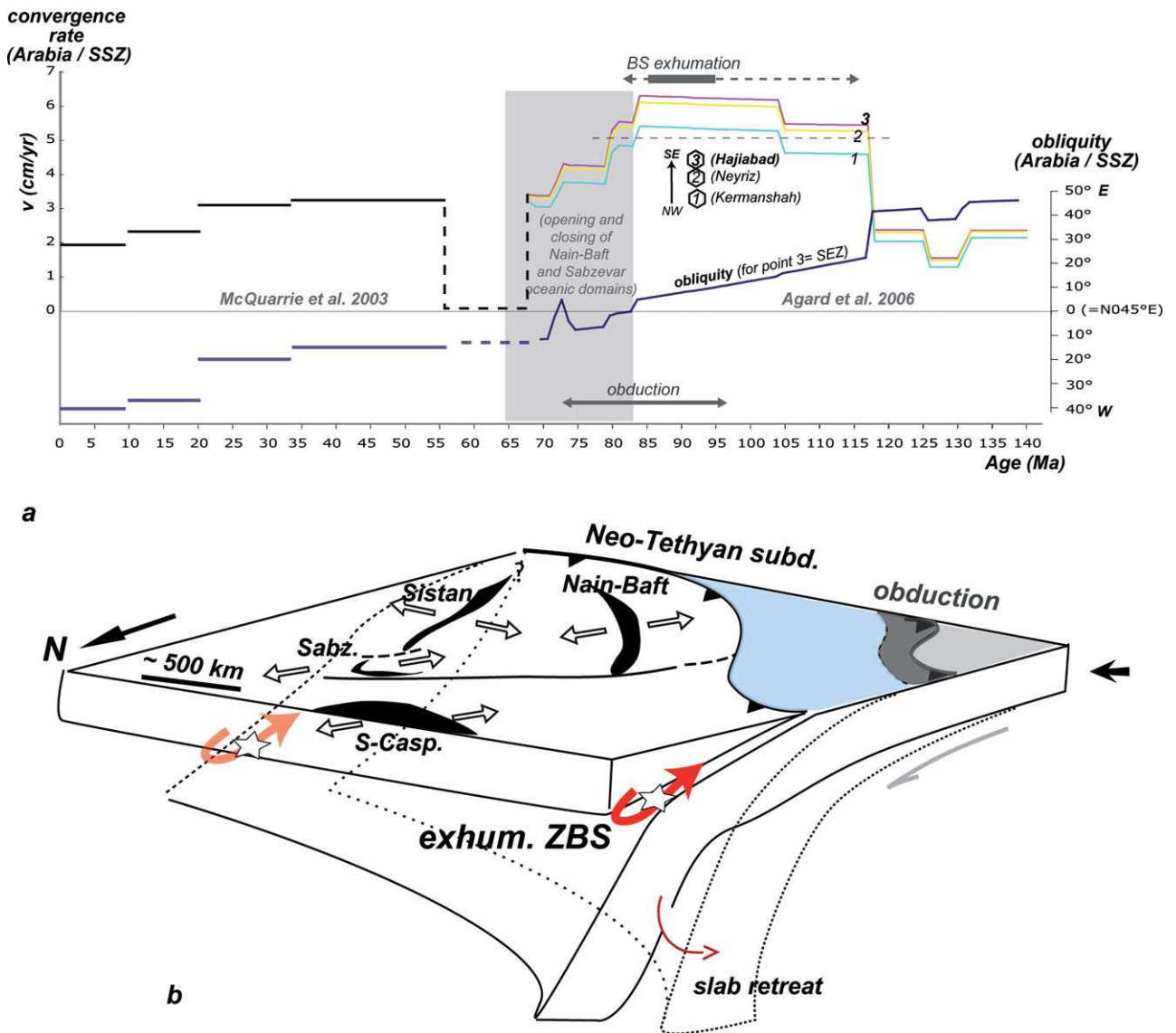
Figure 8. (Colour online) (a) Kinematic constraints for the Zagros convergence. Convergence rates are c. 2\text{--}3 \text{ cm yr}^{-1} on average except for two noticeable periods: (1) a fast convergence period in the Late Cretaceous ( 5\text{--}6 \text{ cm yr}^{-1} ; 118–80 Ma; it coincides, in the region, with obduction and blueschist exhumation); (2) a very slow convergence period in the Paleocene (see also Dewey et al. 1989 and Rosenbaum, Lister & Duboz, 2002). (b) Outline of the specific constraints provided by the almost coincident onset of regional-scale back-arc opening (see Section 3.e), blueschist (BS) exhumation along the Neo-Tethyan subduction zone (red arrows) and obduction onto Arabia following the c. 115 \text{ Ma} kinematic reorganization (a). Situation drawn at c. 90\text{--}85 \text{ Ma} . Stretched, partly oceanic basins formed in the upper plate, from north to south: South Caspian (S-Casp.), Sabzevar (Sabz.), Sistan and Nain–Baft seaways.
