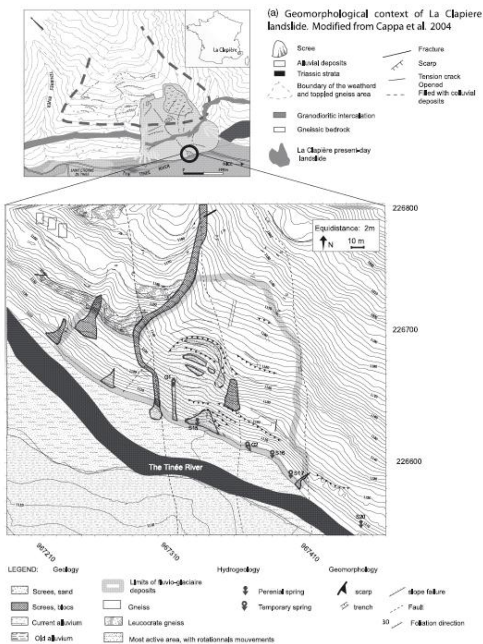
(b) Geomorphological and hydrogeological context of the landslide toes Fig. 1 Localization and topography of the La Clapière landslide (a) and detailed map of the studied secondary encased landslide (b) in the slope toe (from Lebourg et al., 2005).
