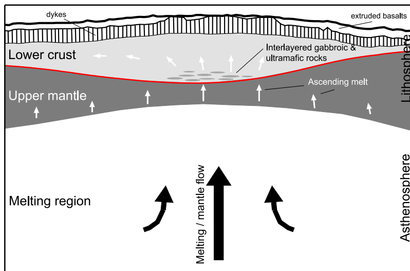
Figure 7. Sketch showing a geological interpretation of our traveltimes modeling. The main features are discussed in the text.
