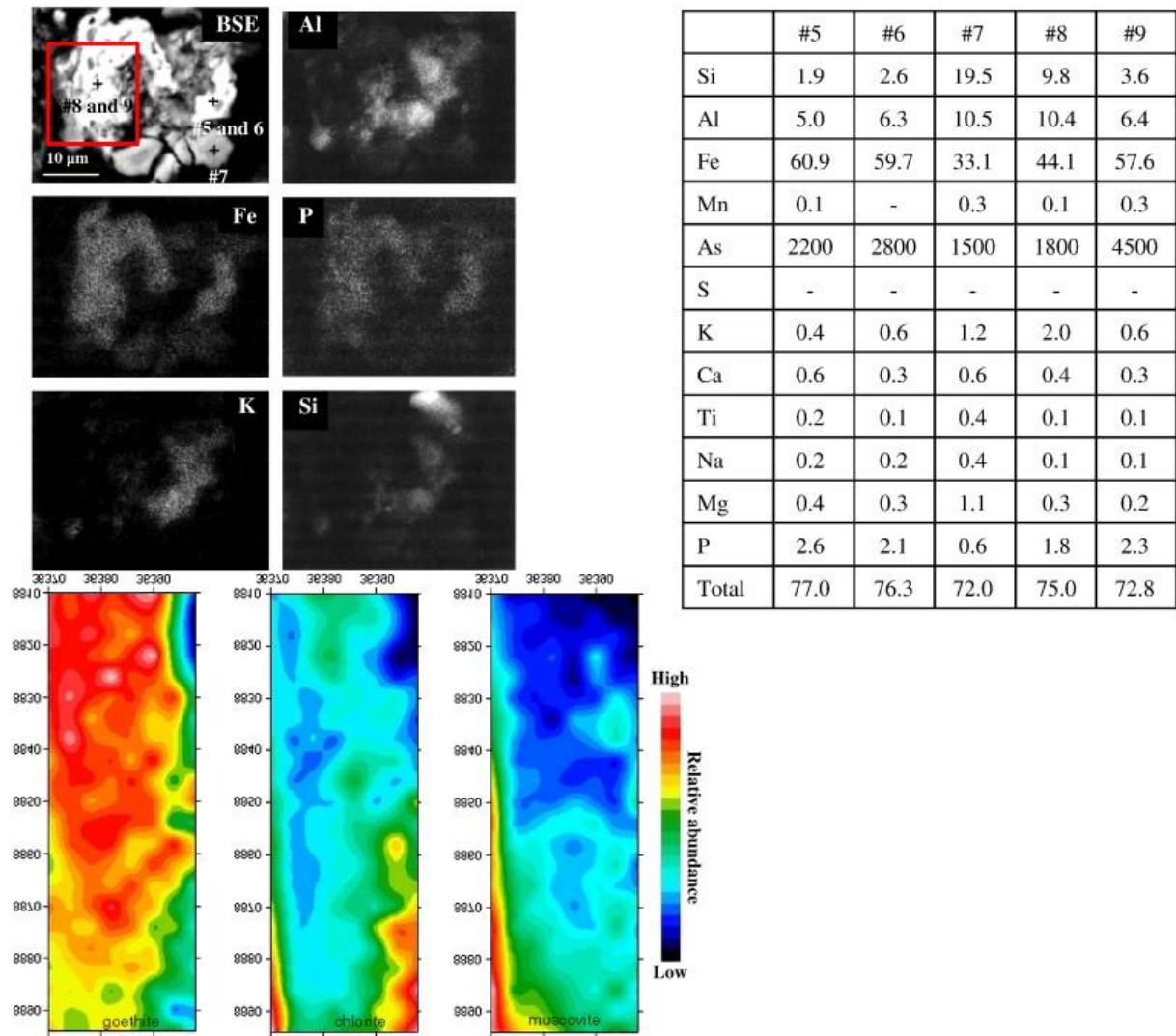
Fig. 4. : BSE microscope image of a representative grain of Fe oxyhydroxide associated to SEM-X ray elemental maps, EPMA analyses and \mu XRD maps corresponding to the square in the particle and representing the distribution of goethite ( 4.18 \text{ \AA} ), chlorite ( 7.07 \text{ \AA} ) and muscovite ( 9.9 \text{ \AA} ) respectively, their main intensity XRD peak. All concentrations are in wt.% except As in mg/kg and total in %.
