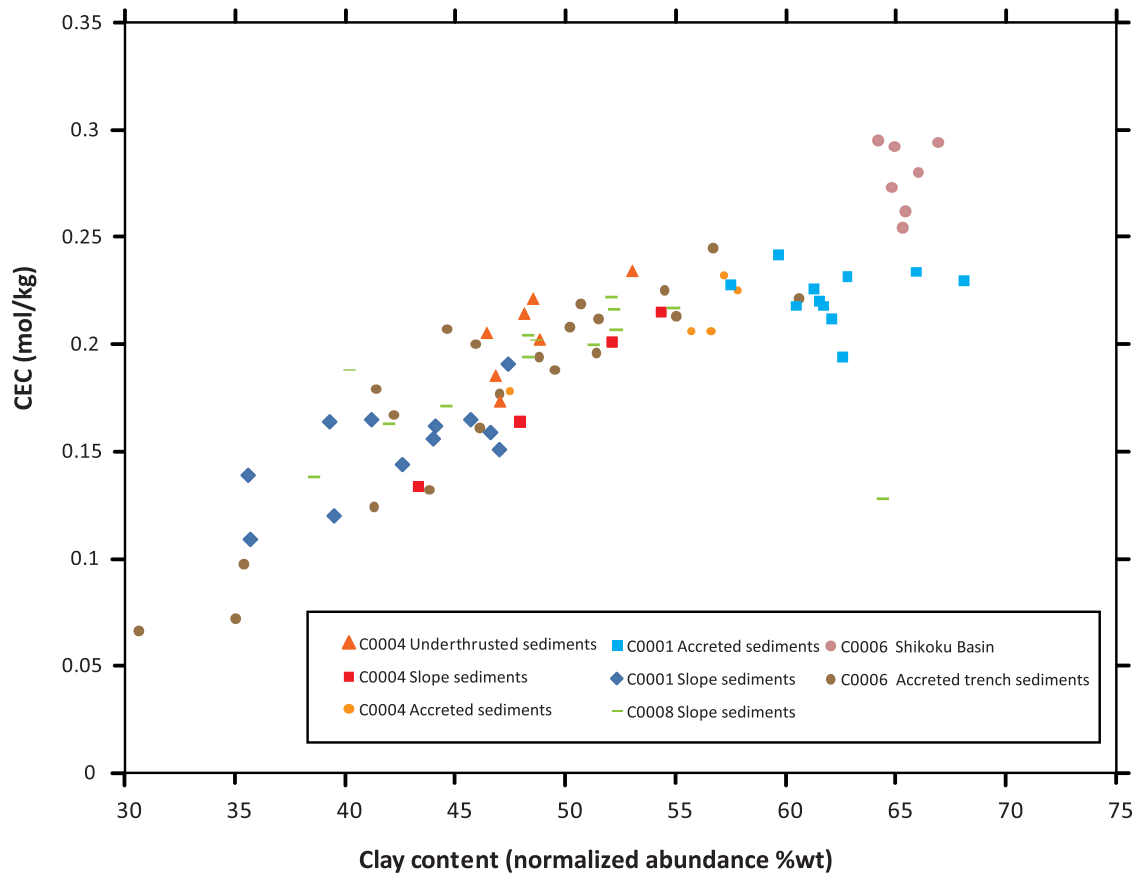
Figure 4. Cation exchange capacity (CEC, in \text{mol kg}^{-1} ) versus normalized abundance of clay mineral content (wt %).
