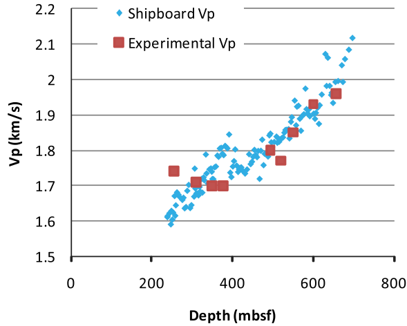
Figure 10. Comparison of compressional velocities V_p either (1) measured onboard on core samples (diamonds), i.e., for P_c = 0 and P_{\text{eff}} = 0 , or (2) estimated in our experiments (squares) as the limit for P_{\text{eff}} = 0 and corrected to P_c = 0 (see text for description). Measurements from both data sets were performed at ambient temperature ( \sim 20^\circ\text{C} – 25^\circ\text{C} ).
