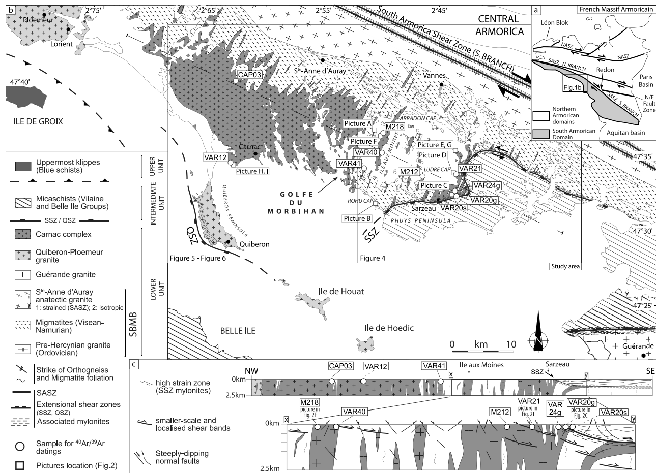
Figure 1. Geological map of the study area and location of the samples used for the ^{40}\text{Ar}/^{39}\text{Ar} analyses. (a) Simplified geological map of the French Massif Armoricain showing the main tectonic domains of the massif. NASZ: North Armorican Shear Zone; SASZ: South Armorican Shear Zone; N. Branch: Northern Branch; S. Branch: Southern Branch; N/E: North-sur-Erdre fault. (b) Detailed map of the studied part of the South Armorican Domain, in the Golfe du Morbihan area. This geological map exhibits the main tectonometamorphic units and their overall internal features. SBMB: South Brittany Migmatite Belt. Geology of Central Armorican domain, north of SASZ is not detailed. South of the SASZ, the Upper Unit cropping out in the Ile de Groix klippe, the Intermediate and the Lower tectonic units are shown. These two latter units are separated by late orogenic extensional shear zones: the Sarzeau Shear Zone (SSZ) in the Rhuy peninsula area and the Quiberon Shear Zone (QSZ) in the Quiberon peninsula area. White squares locate hand-sample and outcrops pictures displayed on Figure 2. White circles locate samples used for the conventional and in situ ^{40}\text{Ar}/^{39}\text{Ar} analyses. Legend for the main geological formations is the same for the map and for the cross sections. (c) Interpretative cross section (dashed line on Figure 1b) through the study area. The structural features of the Golfe du Morbihan-Rhuy peninsula section (noted X-Y) have been detailed. This close-up view shows the different ductile, ductile-brittle and brittle structures described during the structural analysis. Pictures of such structures are reported in Figure 2. Location of samples used for ^{40}\text{Ar}/^{39}\text{Ar} analyses has been projected onto the cross sections.
