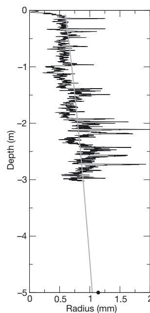
Fig. 5. Snow grain-size profiles obtained using the ADC relationship (black) and derived from Brucker and others (2010) (gray). The dot at 5 m depth corresponds to r^{z>3m} .
