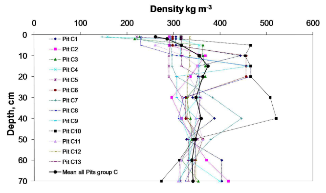
Fig. 5. Density profiles of group C pits at Dome C.
