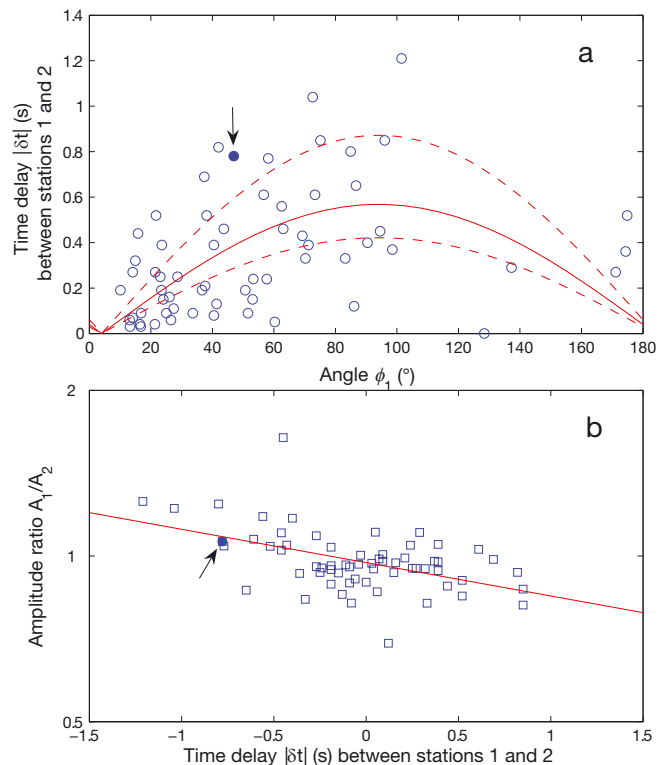
Fig. 7. (a) Distribution of the time delay between stations 1 and 2 vs the polarization angle, \phi_1 , at station 1, for the 63 selected clear LFB arrivals. The best fit (continuous curve) gives v = 1090 \text{ m s}^{-1} , with a standard deviation of 380 \text{ m s}^{-1} (dashed curves). (b) Attenuation in log scale of the LFB wavetrain amplitude between stations 1 and 2 as a function of the time delays, for the same 63 LFBs. The best log-linear fit (continuous line) gives an attenuation of 0.0011 \text{ dB m}^{-1} . The two data points shown by arrows correspond to the 1 min long time window containing the LFB of Figure 5.
