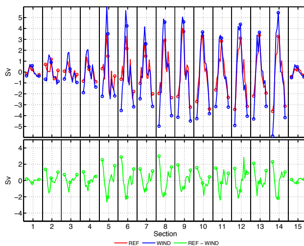
Fig. 12. The upper plot shows the anomaly of monthly ASC transport (compared to the annual mean transport of the ASC shown in Fig. 11) across each section (horizontal axis) shown in Fig. 1. Each number corresponds to one section, and for each section, the circle on the left is January, then June and the circle on the right is December. The blue line is for WIND and the red line for REF. The bottom plot shows the difference between REF and WIND simulations (green line). A negative value means a stronger ASC in WIND simulation.
