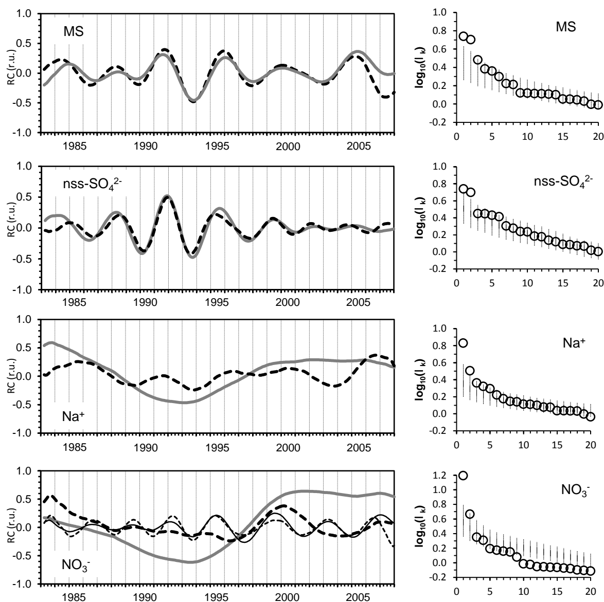
Fig. S3.1. Results from the MC-SSA analyses (embedding dimension: M = 60 ) for monthly anomalies of MS, \text{nss-SO}_4^{2-} , \text{Na}^+ and \text{NO}_3^- measured at NM. Left hand column: Reconstructions based on EOF 1 (bold grey line), EOF 2 (bold dashed black line), EOF 3 (thin black line), and EOF 4 (thin dashed black line). Right hand column: First 20 eigenvalues l_k (circles) of the corresponding EOFs, logarithmic scale. Vertical lines indicate the 95th (upper end) and 5th (lower end) red noise percentiles based on 2000 Monte Carlo simulations.
