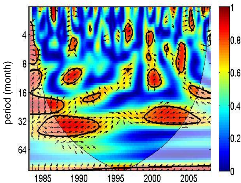
Fig. S3.6. Wavelet coherence between the time series (\text{MS})_{\text{anomaly}} and temperature at 2 m height measured at NM. Description see Figure S3.3.
