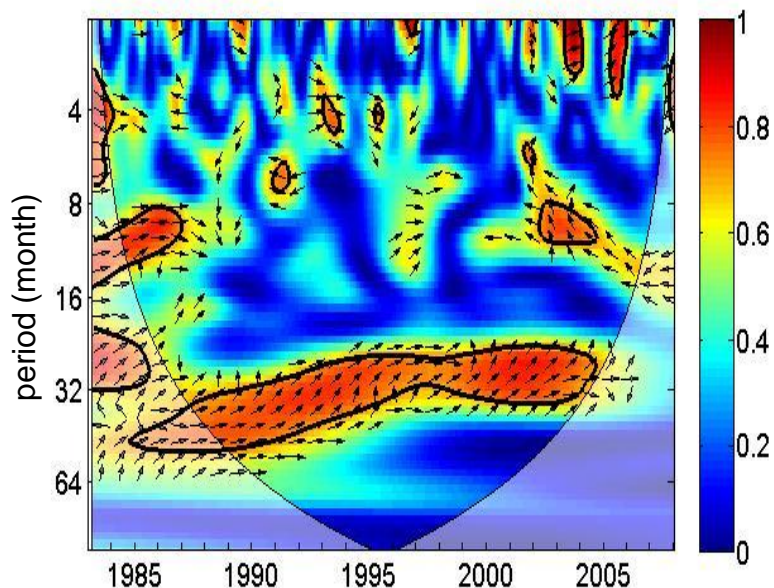
Fig. S3.5. Wavelet coherence between the time series (\text{nss-SO}_4^{2-})_{\text{anomaly}} and temperature at 2 m height measured at NM . Description see Figure S3.3.
