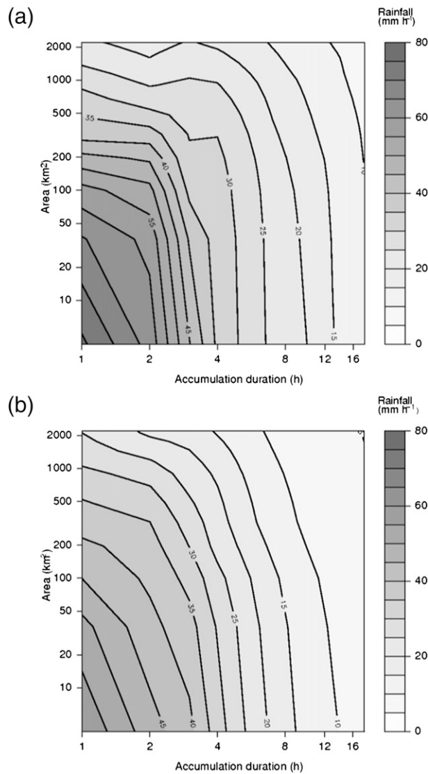
FIG. 8. Maximum intensity diagram for event 2, from 0000 to 1800 UTC 6 Sep 2005 for (a) observed hourly rainfall and (b) simulated rain fields.
