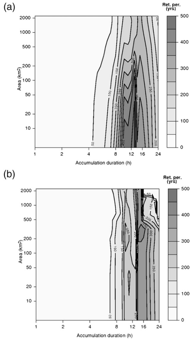
FIG. 10. Severity diagram for event 1, from 0000 UTC 3 Dec to 0000 UTC 4 Dec 2003 for (a) observed hourly rainfall and (b) simulated rain fields.
