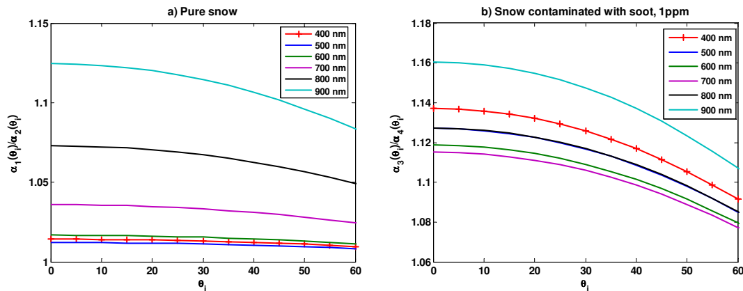
Fig. 3. Ratio \frac{\alpha_1(\theta)/\alpha_2(\theta)}{\alpha_1(\theta)/\alpha_2(\theta)} , for six wavelengths and as a function of the incident zenith angle, \theta_i . (a) Pure snow; (b) snow contaminated with soot (1 ppm).
