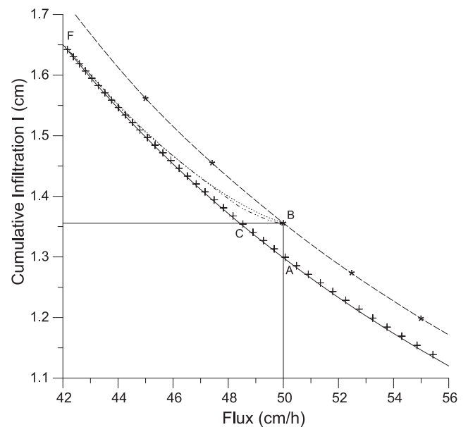
Figure 1. Cumulative infiltration is given as a function of flux, showing the relationship between the cases of q constant and \theta = \theta_{sat} . The dashed line is equation (2) with M neglected, the asterisks give the numerical values, the solid line is equation (20), the crosses give the numerical values, the dashed-dotted line is equation (21) with \alpha = 18.105 , and the dotted line gives the numerical values for the transition from q constant to \theta = \theta_{sat} . BACF is the TCA and BCF is the MTCA.
