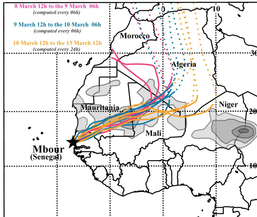
Figure 6. Tri-dimensional air masses back trajectories computed to end at approximately 400 m AGL above the Mbou station during the March 7–13 sampling period. Trajectories' duration varies from 3 days at the beginning of the time series to 6 days toward the end (durations were adapted so that trajectories reached the continent's hedges). Air mass latitude higher than 1500 m (dashed lines) are distinguished from lower transport (solid lines). Calculation was made using the HYSPLIT model (R. R. Draxler and G. D. Rolph, HYSPLIT (HYbrid Single-Particle Lagrangian Integrated Trajectory) Model, 2011, access via NOAA ARL READY Website http://ready.arl.noaa.gov/HYSPLIT.php ; G. D. Rolph, Real-time Environmental Applications and Display system (READY) Website, http://ready.arl.noaa.gov ). Background map shows the annual mean Aerosol Index (AI) values >15 from TOMS data (1980–93, 1997–2000) (adapted from Goudie and Middleton [2001]).
