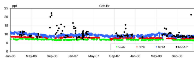
Fig. 7. \text{CH}_3\text{Br} measured at NCO-P (all data) compared with baseline data at MHD (blue), RPB (red) and CGO (green).
