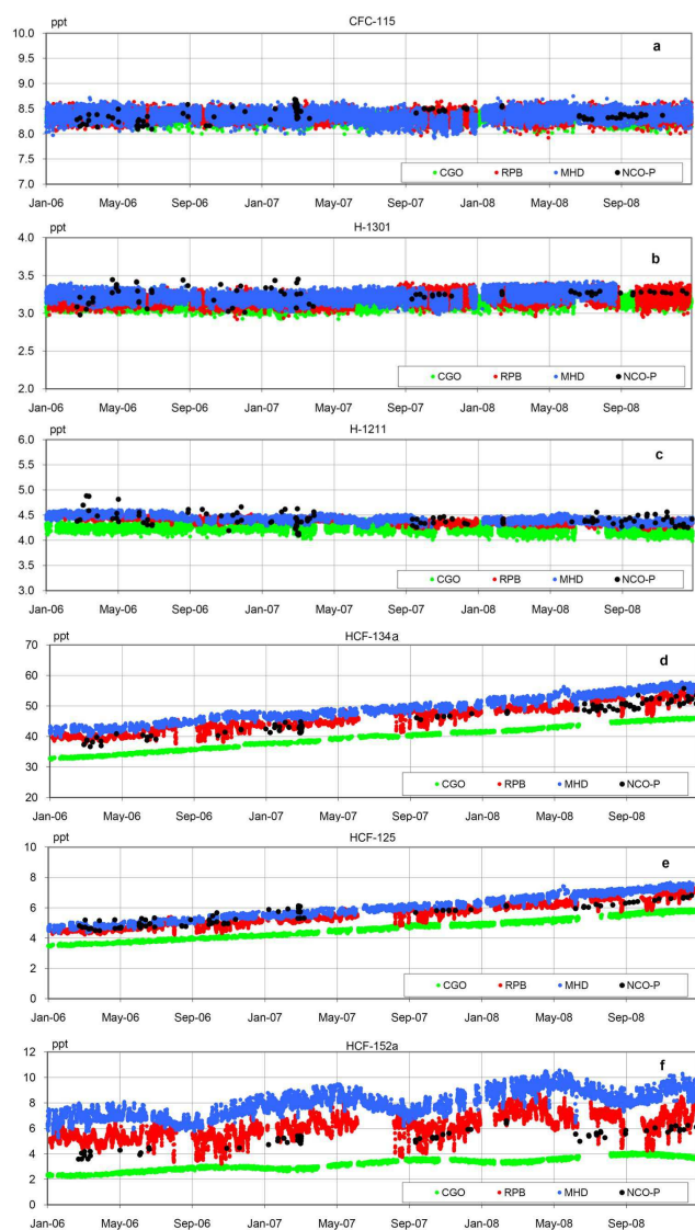
Fig. 5. Meridional gradients: time series for (a) CFC-115, (b) H-1301, (c) H-1211, (d) HFC-134a, (e) HCF-125 and (f) HCF-152 at NCO-P (black) are reported together with those obtained at MHD (blue), RPB (red) and CGO (green). Only baseline data have been considered.
