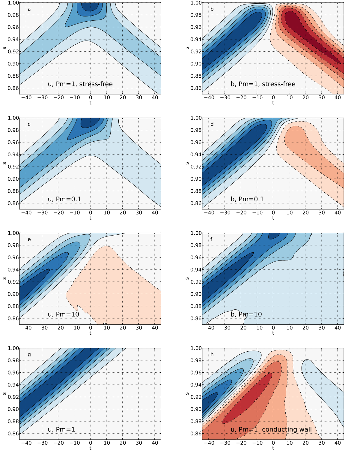
FIG. 4. Space-time diagrams of the reflection of a TAW for S \simeq 10^4 and \ell = 0.02 recorded in the equatorial plane, near the equator. Top row : stress-free boundary with Pm = 1 ( R = 0.88 ), (a) the azimuthal angular velocity u_\phi/s and (b) the azimuthal magnetic field b_\phi (changing sign). Second row : No-slip boundary with Pm = 0.1 ( R = 0.40 ), (c) the azimuthal angular velocity u_\phi/s and (d) the azimuthal magnetic field b_\phi (changing sign). Third row : No-slip boundary with Pm = 10 ( R = -0.17 ), (e) the azimuthal angular velocity u_\phi/s (changing sign) and (f) the azimuthal magnetic field b_\phi . Bottom row : azimuthal angular velocity u_\phi/s for no-slip boundary with Pm = 1 showing no reflection ( R = 0 ) for insulating boundary (g), and little reflection when the insulator is replaced by a solid conductive layer (h).
