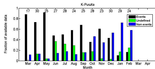
Fig. A8. The fraction of event, undefined and non-event days out of all analyzed days during each month in the year at K-pusztaszeg, Hungary, during March 2008–February 2009.
