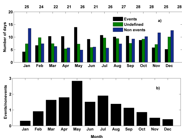
Fig. 4. (a) The median monthly number of particle formation event, undefined and non-event days, and (b) the median monthly event to non-event day ratio for all the sites from April 2008 to April 2009 within the EUCAARI project. The numbers above the top figure refer to the median number of days included in the analysis. These numbers are the average values observed at all the twelve field sites.
