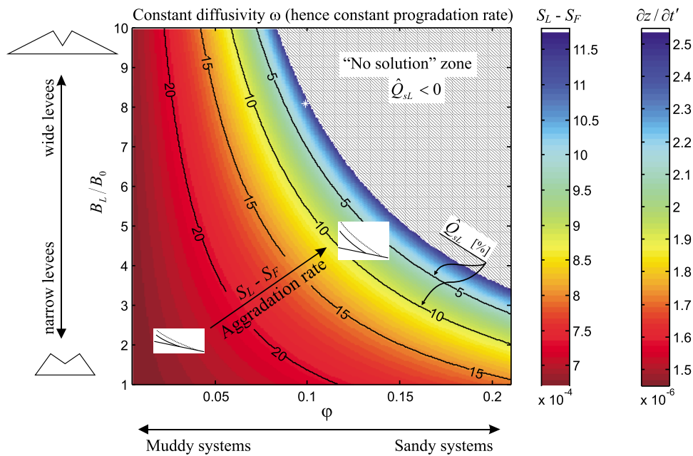
Figure 10. Sensitivity analysis of model behavior. Plot of aggradation rate \partial z/\partial t' = f(\phi, B_L/B_0) for a constant diffusivity ( \omega = 800 \text{ m}^2/\text{s} ) and progradation rate ( \partial L/\partial t' = 2.16 \times 10^{-3} \text{ m/s} ), and other variables fixed as estimated for the Amazon channel in section 5. The white star represents the actual set of model parameters used in the comparison with the Amazon channel presented in section 5.
