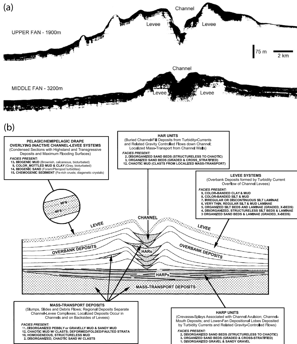
Figure 2. (a) Seismic reflection images of channel cross sections on the Amazon Submarine Fan (redrafted from Damuth and Flood [1985]). Horizontal and vertical bars indicate approximate scale as derived from seismic travel times. (b) Schematized evolution of a leveed channel on the Amazon Submarine Fan, showing the distribution of sedimentary facies within acoustic units (e.g., HAR units, HARP units) and turbidite elements (e.g., channel, levee/overbank, mass transport deposits (MTDs)) of the Amazon Fan. A typical channel-levee system is shown, which is the elemental stratigraphic unit of the fan, and an underlying regional-scale MTD. This stratigraphic relationship is typical of the upper and middle fan [Damuth et al., 1988]. Lower fan deposits lack large channel-levee systems and, for the most part, consist of depositional lobes containing facies comparable to those of the HARP units described in this diagram. From Normark et al. [1997]. MFS, maximum flooding surface.
