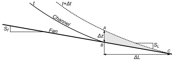
Figure 5. Channel aggradation and subsequent progradation of the channel downstream tip on the surrounding unchannelized fan.
