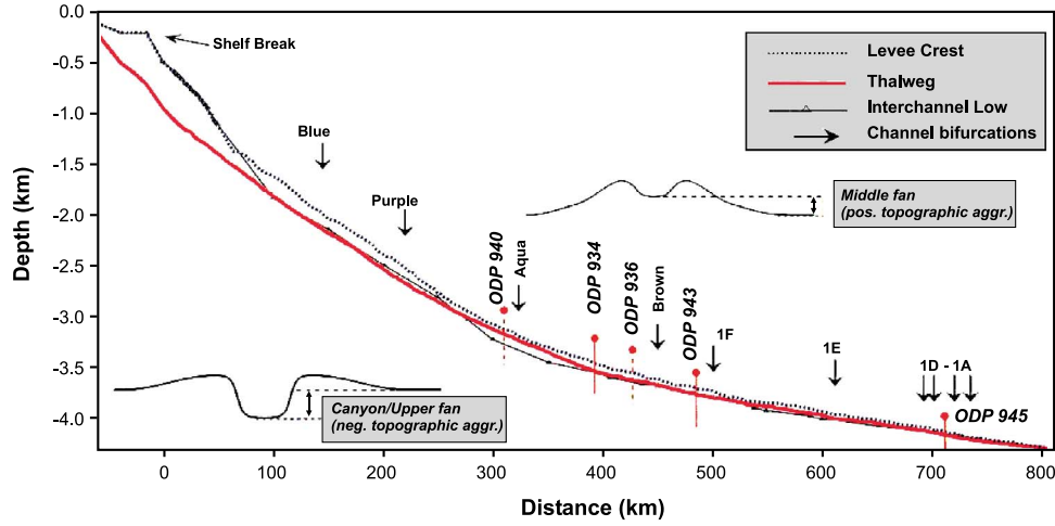
Figure 3. Long profile of the main channel of the Amazon Submarine Fan [from Pirmez and Imran, 2003] (with permission from Elsevier).
