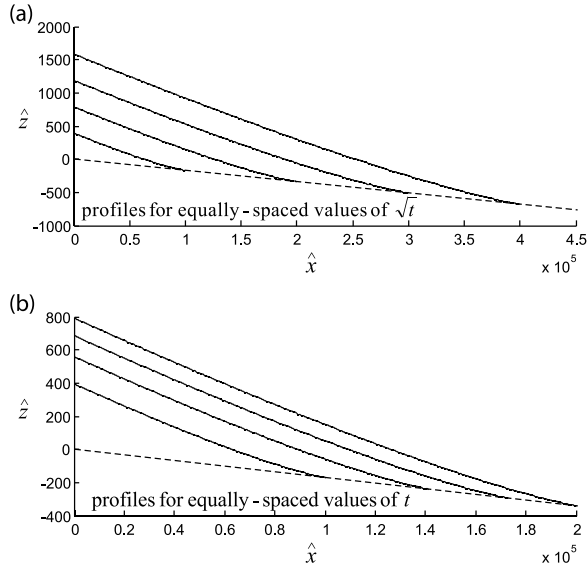
Figure 6. Self-similar evolution of the channel long profile (solid lines) as it aggrades and progrades on the surrounding fan (dashed line): (a) profiles at equidistant intervals of channel length L(t') = \sqrt{2\omega t'} ; and (b) profiles at equidistant intervals of time t' . The value of n used in the calculation was 0.4.
