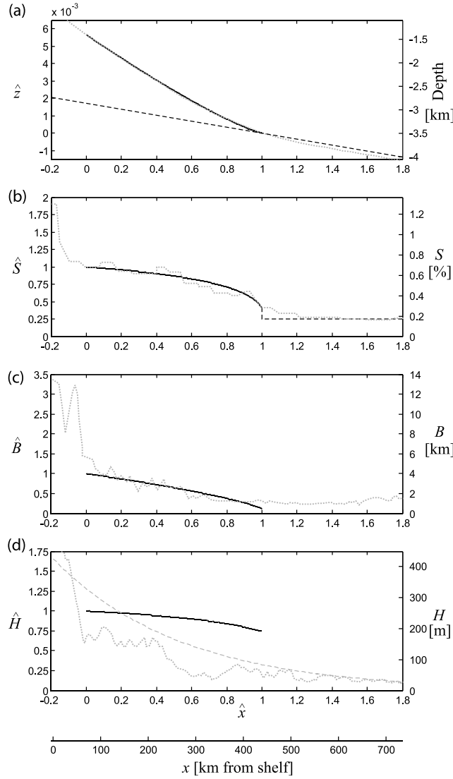
Figure 7. Comparison of model predictions (black curves) with actual data (gray dotted curves) of the Amazon submarine channel, for several meaningful morphological variables: (a) channel long profile, with the modeled surrounding fan plotted as the dashed black segment; (b) channel slope; (c) channel bankfull width; (d) channel relief, with the dashed gray curve representing the age-corrected exponential fit proposed by Pirmez and Imran [2003]. All scales are presented in dimensionless similarity variables on the left axis, as well as dimensional metric variables on the right axis. On the horizontal axis, actual downstream distance from the shelf edge is plotted in addition to dimensionless distance \hat{x} , with model results spanning over \hat{x} = 0 to 1. The more upstream reaches correspond to the incised canyon, and the more downstream reaches correspond to the modern, poorly channelized lower channel below the Brown paleoavulsion site.
