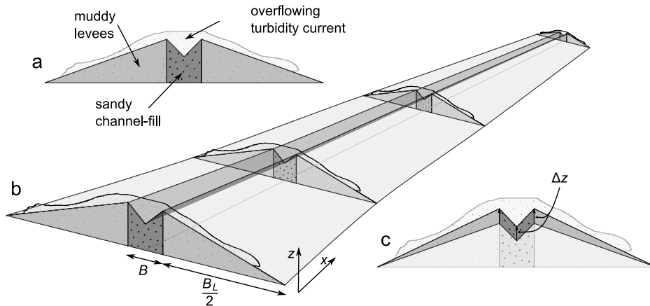
Figure 4. Schematization of the assumed simplified architecture of the channel-levee system. (a) Triangular cross section with a sandy channel fill and muddy levees; (b) axonometric view illustrating a downslope reduction in channel width and relief; and (c) channel buildup by concurrent aggradation of the bed and levees. The channel is illustrated as straight only for simplicity.
