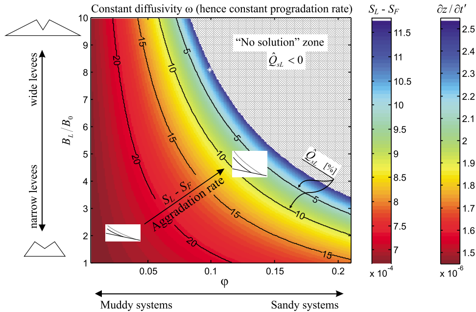
Figure 10. Sensitivity analysis of model behavior. Plot of aggradation rate \partial z / \partial t' = f(\phi, B_L / B_0) for a constant diffusivity ( \omega = 800 \text{ m}^2/\text{s} ) and progradation rate ( \partial L / \partial t' = 2.16 \times 10^{-3} \text{ m/s} ), and other variables fixed as estimated for the Amazon channel in section 5. The white star represents the actual set of model parameters used in the comparison with the Amazon channel presented in section 5.
