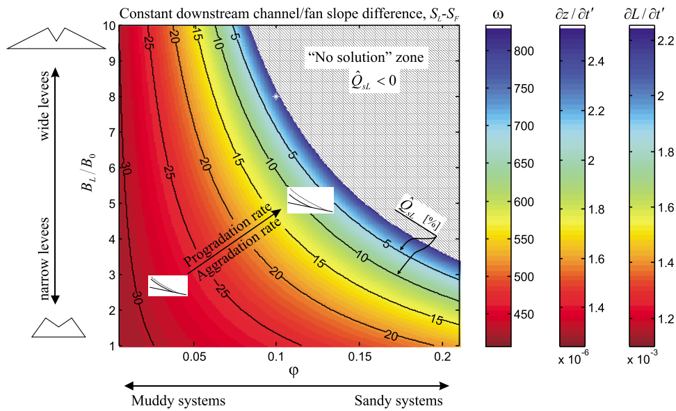
Figure 9. Sensitivity analysis of model behavior. Plot of effective diffusivity \omega = f(\phi, B_L/B_0) for a constant downstream channel/fan slope difference, S_L - S_F , with other variables fixed as estimated for the Amazon channel in section 5. The white star represents the actual set of model parameters used in the comparison with the Amazon channel presented in section 5.
