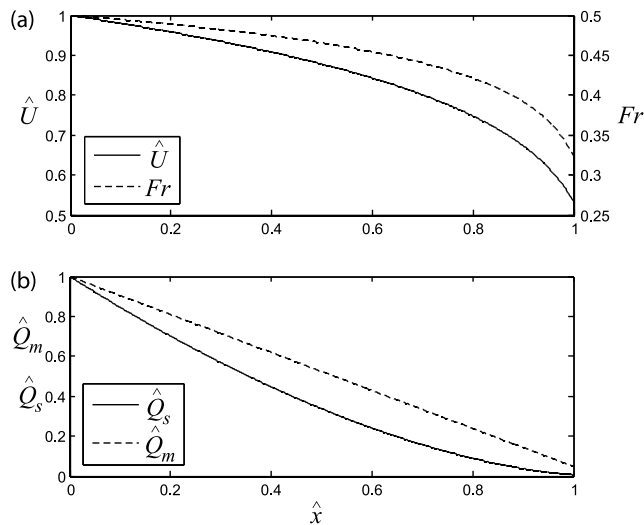
Figure 8. Model predictions for the long profiles of sediment discharges and flow characteristics associated with channel-forming turbidity currents in the Amazon submarine channel: (a) cross-section-averaged current velocity and densimetric Froude number; and (b) sand and mud discharges of sediment suspended in the flow. All plots are presented in dimensionless similarity variables.
