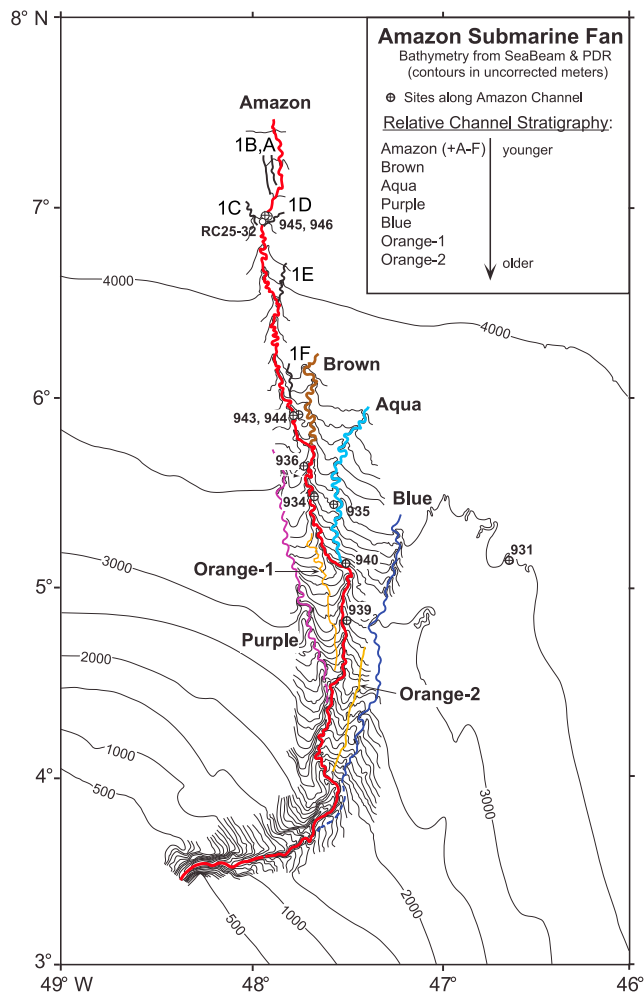
Figure 1. Planform of the Amazon Submarine Fan [from Pirmez and Imran , 2003] (with permission from Elsevier), indicating the latest elongated Amazon channel as well other antecedent paleochannels and ODP core sites.
