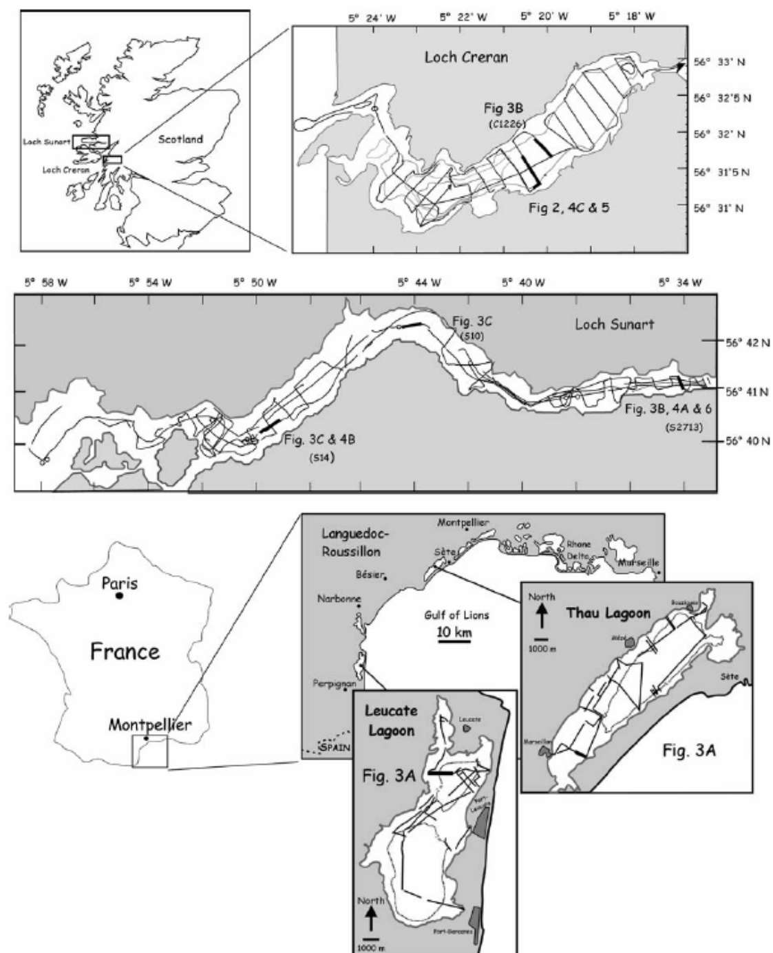
Figure 1. Location of the different study areas and Seistec profiles acquired in Scotland (Loch Sunart and Loch Crenan) and France (Lake Leucate and Thau Lagoon)
