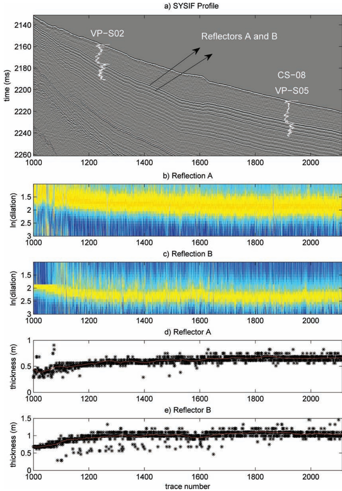
Figure 9. (a) Seismic profile across a submarine landslide in HR (220–1050 Hz) domain, in situ P-wave velocity profiles (VP-S02 and VP-S05), CS-08 core sample location and A and B seismic reflectors pointed with black arrows. (b and c) Ridge function attributes of reflectors A and B , respectively, as a function of the seismic trace number. (d and e) Reflector thicknesses extracted from the ridge function attributes. Note that both thicknesses increase from the upper part to the base of the landslide with a super-resolution.
