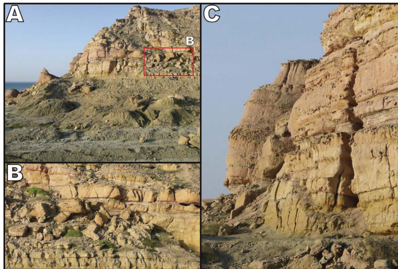
Figure 2. “Disputed” outcrops. (a) Locality illustrated by Bourgois et al. [2007, Figures 5A and 9], immediately to the NE of Cabo Blanco. The car in the middle right of the photograph gives the scale. (b) Close-up of the “notches” which we interpret as resulting from differential erosion of beds of different lithologies. (c) Frontal view of the base of the cliff, with subhorizontal bedding of the Talara formation which induced Bourgois et al. [2007] to erroneously consider that the erosion notches were produced by successive stands of sea level in the latest Quaternary. (Photos L. Ortlieb, May 2010.)
