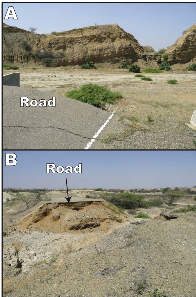
Figure 1. Examples of road and bridge destructions along the Panamerican highway-related to strong rainfalls (a) East of Talara; (b) Southeast of Cabo Blanco. Most of these destructions resulted from floods that occurred during the last very strong El Niño event of 1997–98. (Photos L. Ortlieb, May 2010.)
