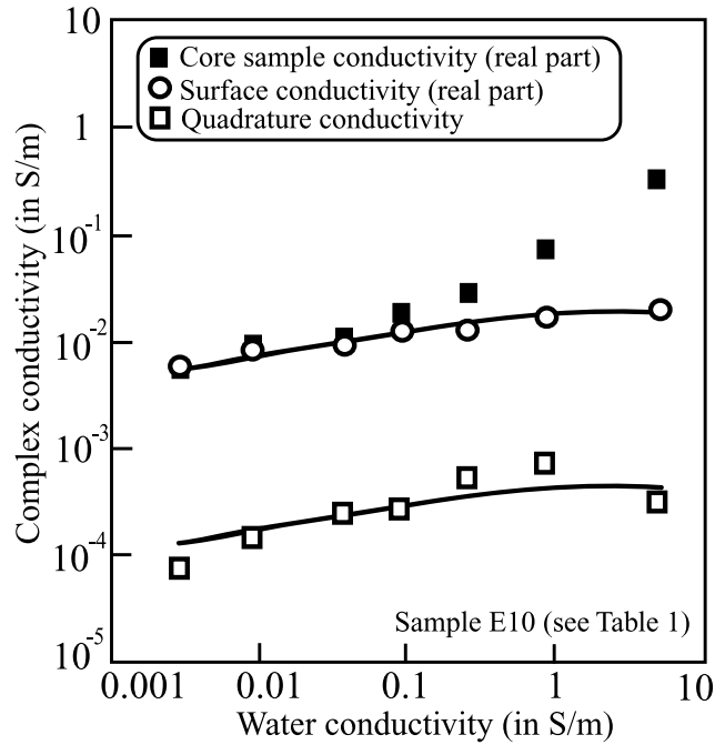
Figure 2. Experimental data showing the salinity dependence of the in phase conductivity, the surface conductivity contribution to the in-phase conductivity and the quadrature conductivity for a sandstone (modified from Börner 1992). Note that the salinity dependence of surface conductivity and quadrature conductivity seems to be the same. This may mean that the same process is at play. This process can only be understood in terms of fundamental electrochemistry of the electrical triple layer coating the pore water mineral interface. The solid lines are just guides for the eyes.
