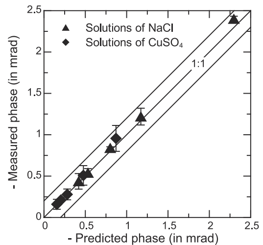
Figure 12. Comparison between the measured phase and the phase predicted with the model shown in this paper for 10 electrolytes at 183 mHz. The triangles correspond to the solutions of NaCl with conductivities of 100, 210, 320, 420, and 550 \mu\text{S cm}^{-1} , respectively (at 25°C). The diamonds correspond to the solutions of CuSO 4 with conductivities of 110, 210, 320, 410, and 510 \mu\text{S cm}^{-1} , respectively.
